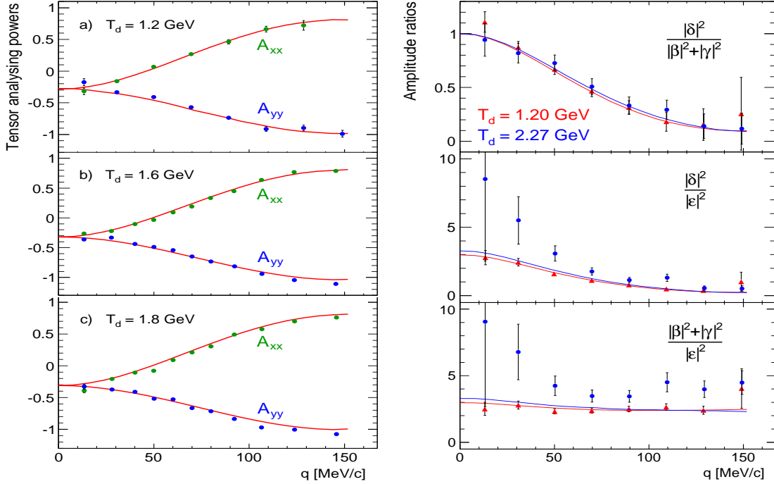
Figure 1: Left panel: Cartesian tensor analysing powers A_{xx} (green dots) and A_{yy} (blue dots) of the \vec{d}p \rightarrow \{pp\}_s n reaction at beam energies of T_d = 1.2, 1.6, and 1.8 GeV for low diproton excitation energy, E_{pp} < 3 MeV. The solid red curves are results of an impulse approximation calculation, where the input np amplitudes were taken from the SAID program at the appropriate energies. Right panel: measured observable ratios as functions of q for two different beam energies. Solid lines are impulse approximation predictions.
