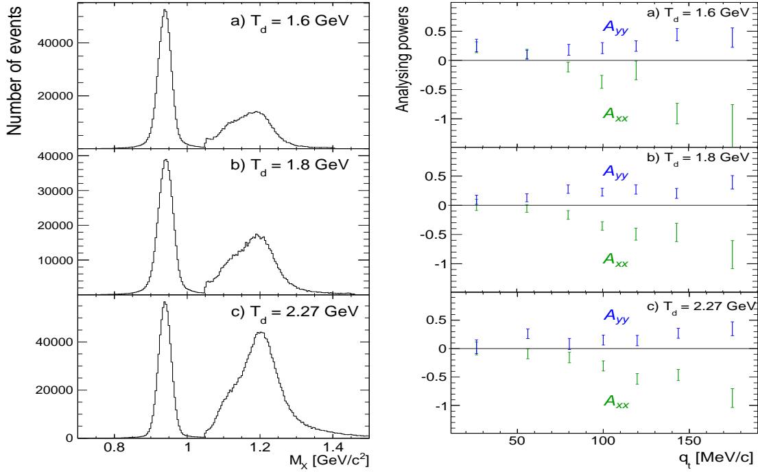
Figure 2: Left panel: The missing-mass M_x distribution for the reaction \vec{d}p \rightarrow \{pp\}_s n at three deuteron beam energies. In addition to the neutron peak, one sees clear evidence for the excitation of the \Delta^0 isobar. (The data in the high mass region have been scaled up by factor of eight.) Right panel: A_{xx} and A_{yy} tensor analysing powers at three deuteron beam energies. Higher mass region is used only.
