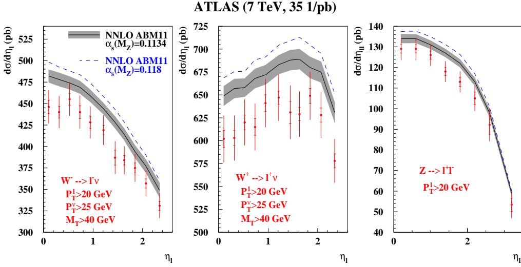
Figure 4: The ATLAS data of Ref. [17] on the rapidity distribution of the charged leptons l^- (left panel), l^+ (central panel), and Z-boson (right panel) in comparison with the NNLO predictions computed with the ABM11 PDFs taking into account the uncertainties due to PDFs (shaded area). The dashed curves display the ABM11 predictions obtained with the value of \alpha_s(M_Z) = 0.118 .
