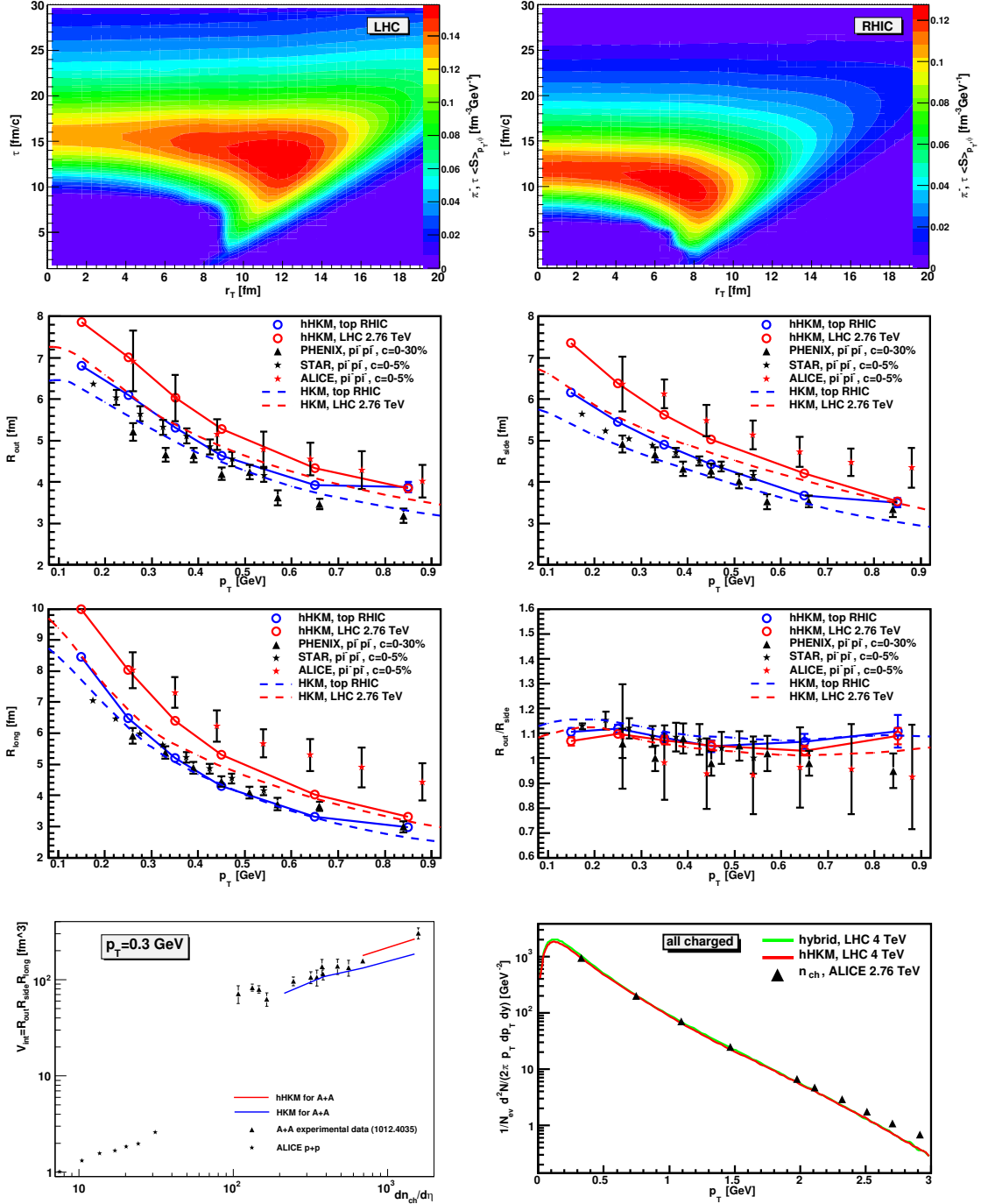
Figure 1: The p_T -integrated emission functions of negative pions for the top RHIC and LHC energies in hHKM(top); the interferometry radii and R_{out}/R_{side} ratio (middle); the transverse momentum spectra of all charged pions at the LHC energy 2.76 TeV in hHKM model, and multiplicity dependence of the pion interferometry volume for central heavy ion collisions at AGS, SPS, RHIC and LHC energies in comparison with the results in p+p collisions (bottom). The solid lines connect the points obtained within HKM and hHKM. The experimental data for A+A collisions are taken from [8, 16, 17, 18, 19, 20, 21, 22]. For p+p collisions at LHC the points for p_T = 0.3 GeV are interpolated from the results of Ref. [23].
