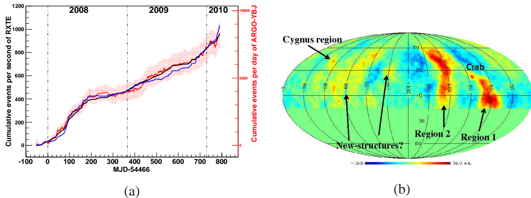
Figure 6: (a): Mrk421 long-term monitoring by the ARGO-YBJ experiment. The vertical axis reports the cumulative number of ARGO-YBJ events (red band, statistical error only), together with two correlated cumulative distributions of X-ray emission. (b): Medium scale anisotropy observed by the ARGO-YBJ experiment. An equatorial representation of data is provided. The color scale indicates the statistical significance of the observation.
