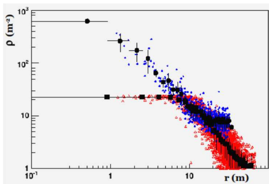
Figure 4: Example of inter-calibration of the digital and the analog information within the same event.
