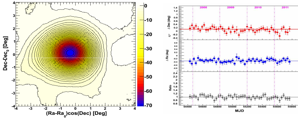
Figure 3: Moon shadow as observed by the ARGO-YBJ experiment (left plot). The color scale indicates the significance of the detection in standard deviations. The right plot reports some results about the operational stability of ARGO-YBJ, carried out on a monthly basis. The deviation of the Moon signal from the expected position in declination (red) and right ascension (blue points) is reported. The black points indicate the ration of the measured signal intensity to the expected one.
