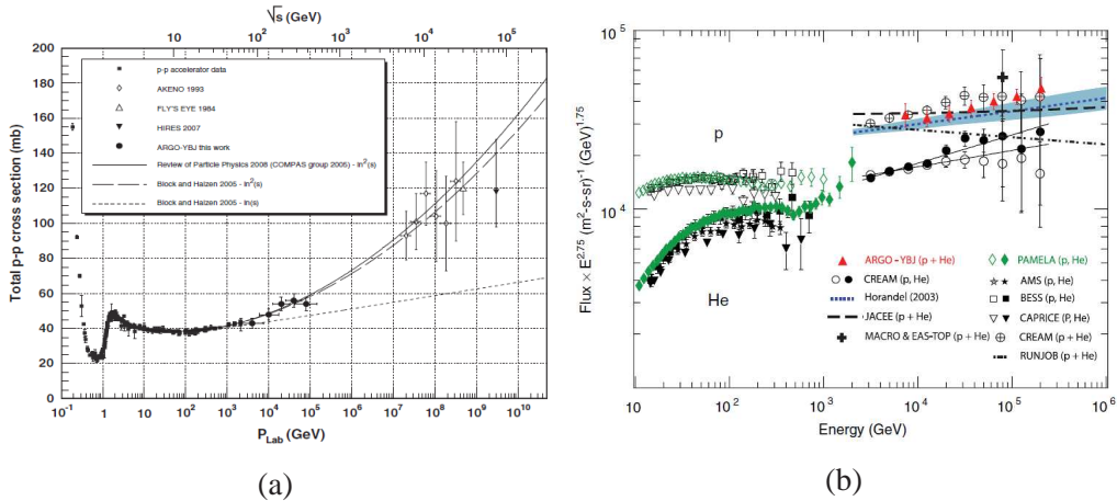
Figure 5: (a): p-p total cross-section measured by the ARGO-YBJ experiment. LHC experiments confirmed in the last year. (b): light component (p+He) energy-spectrum as measured by ARGO-YBJ. Heavier elements amount to a few percent of the data-set and can be reliably excluded from the analysis by suitable selection cuts.
