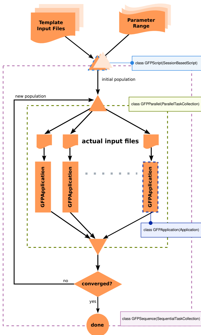
Figure 1: The GFPremium workflow
