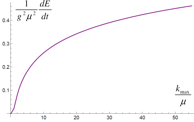
Figure 1: The parton energy loss per unit time in equilibrium plasma as a function of \frac{k_{\max}}{\mu} .
