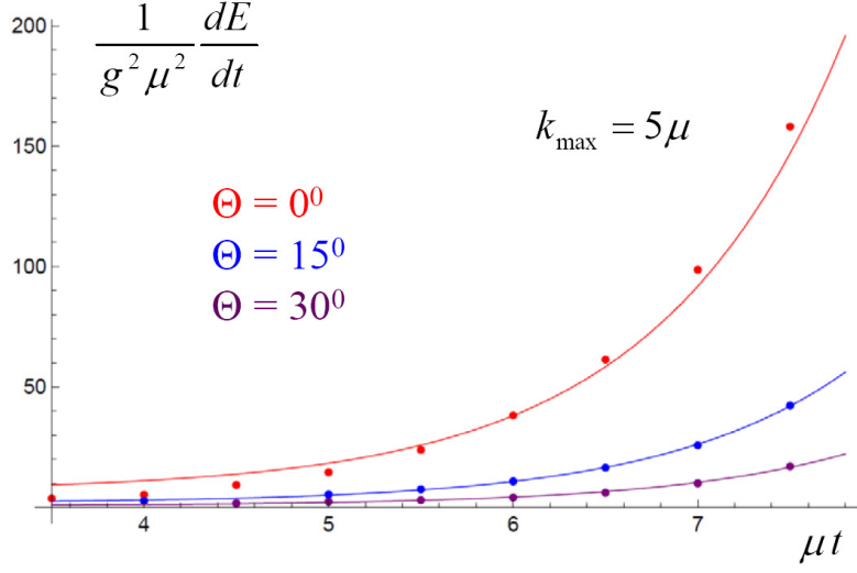
Figure 2: The parton energy loss per unit time as a function of time for three angles \Theta between the parton's velocity \mathbf{v} and the axis z . The red points correspond to \Theta = 0 , the blue ones to \Theta = \pi/12 and the purple points to \Theta = \pi/6 . The solid lines represent the exponential fits to the computed points.
