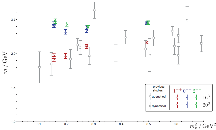
Figure 2: Lattice QCD predictions for exotic isovector mesons [6].
