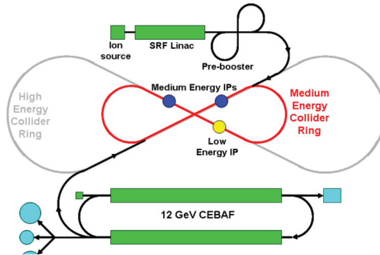
Figure 6: A schematic drawing of MEIC. The high energy ring is a future possibility.
