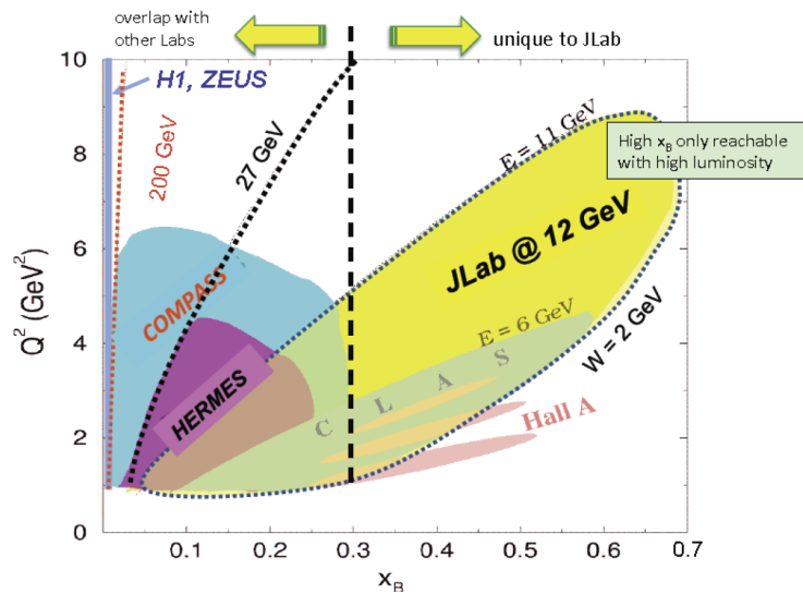
Figure 4: Kinematic reach of the 12 GeV upgrade at Jefferson Lab in Q^2 and x space, in relation to other previous facilities and experiments [4]. The higher energy, combined with the higher luminosity available at JLab, offers new opportunities to explore nucleon structure in the valence quark regime.
