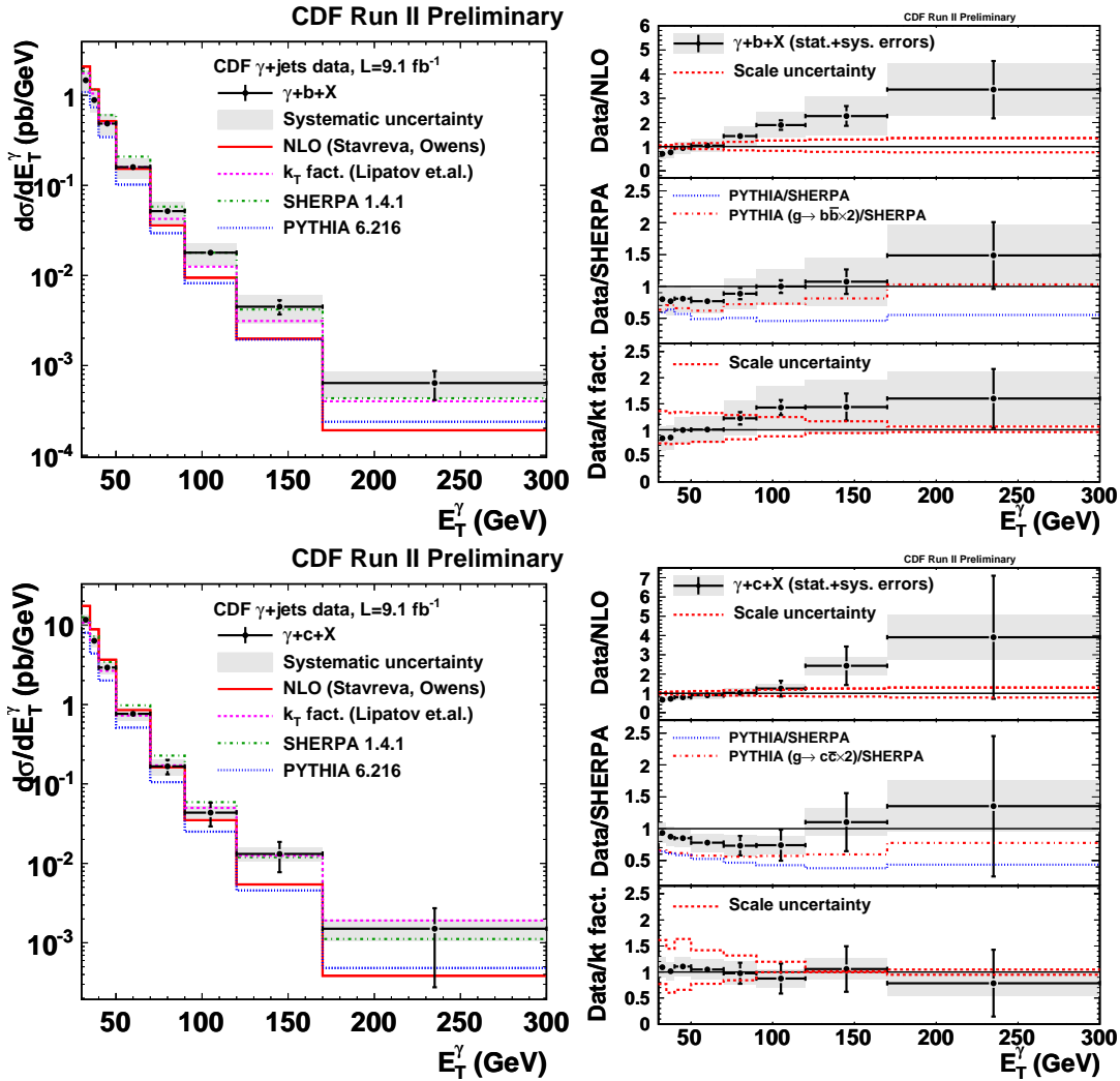
Figure 1: Differential cross sections and data/theory ratios for photon+heavy flavor production. The shaded band shows the total systematic uncertainty of the measurement.
