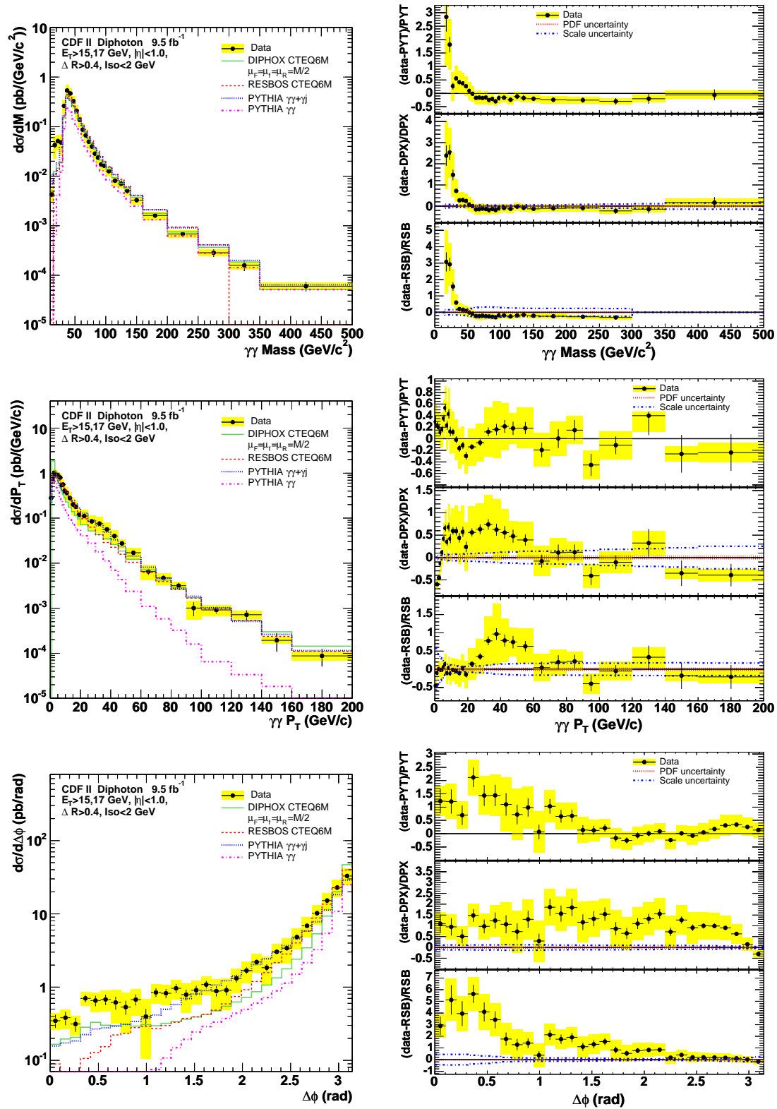
Figure 2: Differential cross sections and (data–theory)/theory ratios for diphoton production. The shaded band shows the total systematic uncertainty of the measurement.
