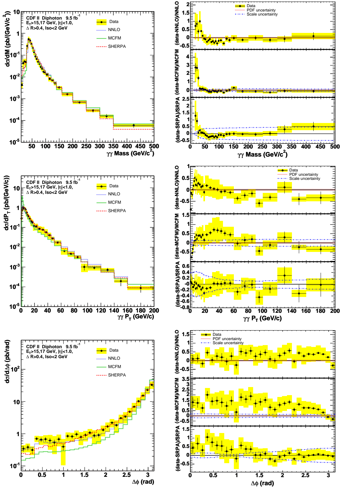
Figure 3: Differential cross sections and (data–theory)/theory ratios for diphoton production. The shaded band shows the total systematic uncertainty of the measurement.
