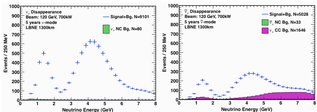
Figure 4: The expected spectra for oscillated \nu_\mu events in neutrino mode (left) and anti- \nu_\mu events in antineutrino mode (right) for a 34 kton LAr TPC at 1300 km in 5 years of running in a 700 kW beam assuming normal mass ordering, \Delta m_{32}^2 = 2.35 \times 10^{-3} \text{ eV}^2 , and \sin^2 2\theta_{13} = 0.1 . Backgrounds from neutral current events (NC) in both modes and neutrino contamination or wrong-sign neutrino events (CC) in antineutrino mode are also shown. The bimodal oscillation pattern is clearly visible at these large distances.
