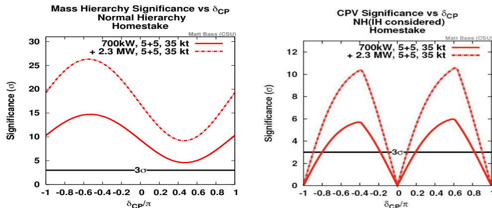
Figure 3: Mass hierarchy and CP violation reach in LBNE for a 35 kton (fiducial mass) detector running for 5+5 years of neutrino+antineutrino running in the standard 700 kW LBNE beam (solid curves) and with the addition of 5+5 years of running with a 2.3 MW beam upgrade made possible with Project X (dashed curves). Both plots assume a \sin^2 2\theta_{13} value of 0.095.
