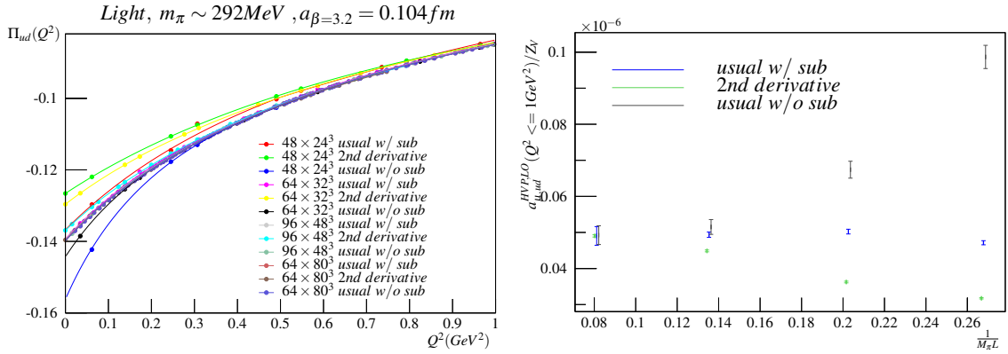
Figure 1: (Left panel) \Pi_{ud}(Q^2) vs Q^2 for M_\pi \sim 292\text{MeV} , as obtained using the usual and 2nd derivative (Eq. (2.5)) methods in four volumes and with all other lattice parameters fixed. The data points are the values obtained from the current-current correlation function and its Fourier derivatives. The curves are the corresponding fits. (Right panel) a_{\mu,ud}^{\text{HVP,LO}}(Q^2 \leq 1\text{GeV}^2) vs 1/M_\pi L obtained from the polarization functions in the left panel.
