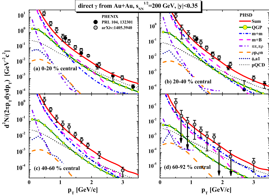
Figure 3: Contribution of the photon production in the two-to-two \rho +nucleon interaction (orange dash lines) to the total direct photon spectra (red lines) at the top RHIC energy of \sqrt{s_{NN}} = 200 GeV at different centralities. The dominant sources are the photons from the QGP and from the hadronic two-to-three bremsstrahlung processes. The theory lines – except the \rho +nucleon channel – are taken from the PHSD predictions published in [7]. The PHENIX data are from Ref. [20, 21].
