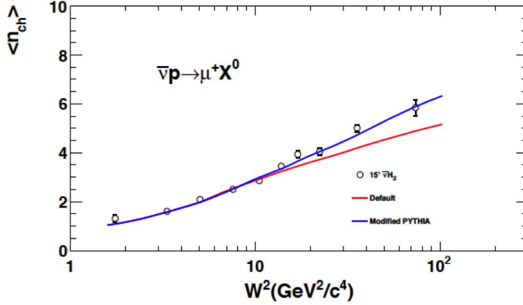
Figure 3: (color online) Averaged charged hadron multiplicity plot. Here, two predictions from GENIE are compared with bubble chamber \bar{\nu}_\mu - p hadron production data [24].
