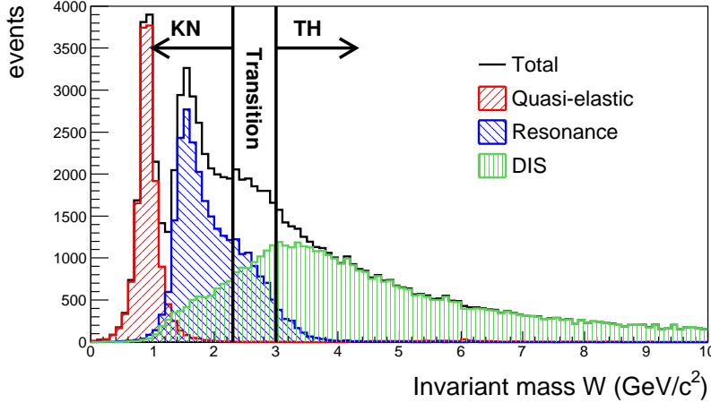
Figure 1: (color online) W distribution of \nu_\mu -water target interaction in GENIE. For the flux, we use an atmospheric \nu_\mu neutrino spectrum. Left red hatched region is quasi-elastic scattering, middle hatched region is resonance interactions, and right green hatched region is from DIS. The W distribution can be splitted to three regions, KNO scaling-based model only region, PYTHIA only region, and the transition region.
