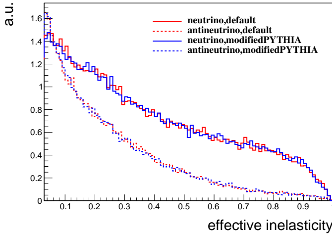
Figure 4: (color online) Effective inelasticity distribution with atmospheric neutrino spectrum. Here, all histograms are arbitrarily normalized. Solid histograms are muon neutrino distributions, and dashed histograms are muon anti-neutrino distributions. Red histograms are from GENIE with the default hadronization model, and blue histograms are from GENIE with the modified hadronization model discussed in this paper.
