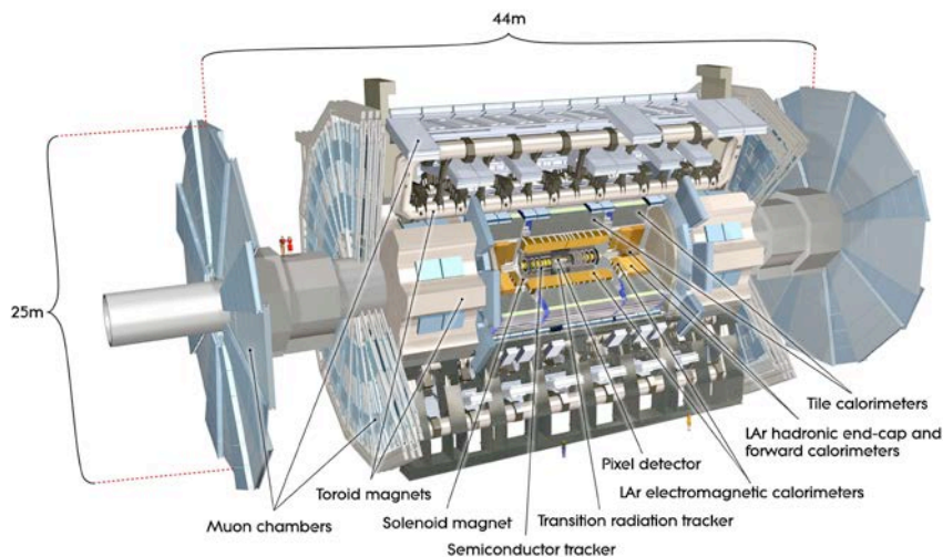
Figure 3: The ATLAS detector with its most important components. ATLAS has a length of 44 m, a diameter of 25 m and registers information from about 90 million individual sensors.
