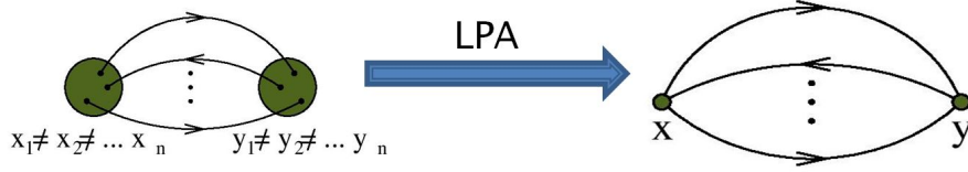
Figure 1: The effect of the local potential approximation: at a certain scale the vertex appears as a point ( left ), below this scale we can think of it as a patch of very close points ( right ).
