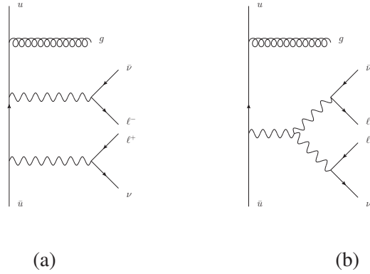
Figure 1: Sample diagrams entering the calculation of the leading order amplitude for the WW + jet process, corresponding to (a) W emission from the quark line and (b) emission from an intermediate Z boson or photon.
