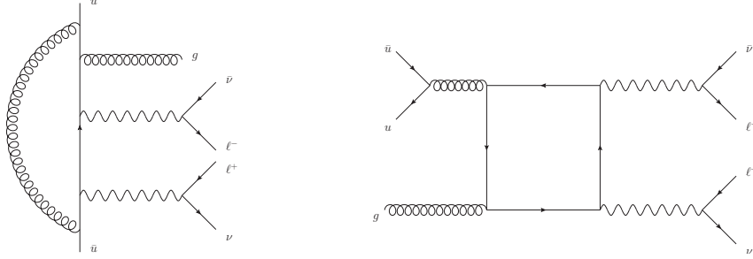
Figure 2: Sample diagrams entering the calculation of the one-loop amplitude for the WW+jet process. The one-loop diagrams can be categorized according to whether a gluon dresses a leading-order amplitude (left), or whether the diagram includes a closed fermion loop (right).
