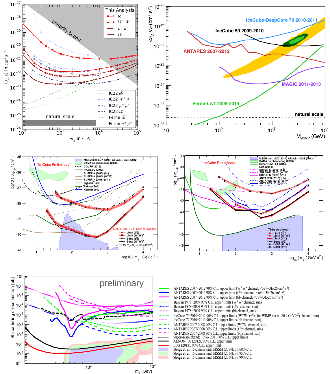
Figure 12: A collection of current neutrino bounds on Dark Matter. First line: bounds on DM annihilations in the Galactic Halo (left, figure from ICECUBE [121]) or the Galactic Center (right, figure from ANTARES [122], referring to the \tau^+\tau^- channel). Notice that the left figure assumes a NFW profile renormalized with a local density of 0.47 \text{ GeV}/\text{cm}^3 while the right one assumes 0.4 . Second line: bounds on the DM scattering cross section with nucleons, from DM accumulated in the center of the Sun, obtained by ICECUBE (left: figure from [115], for the Spin Dependent case; right: figure from the parallel analysis in [116], for the Spin Independent case). Third line: bounds on the SI cross section from DM in the center of the Earth (figure from [117]).
