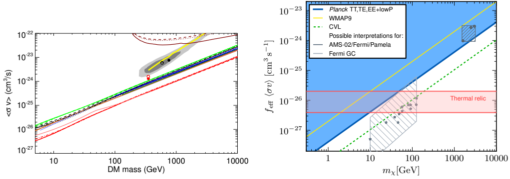
Figure 4: CMB bounds on DM annihilation (figures from [31] and [1]).
