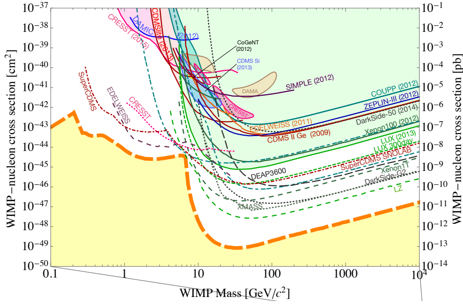
Figure 14: Status of Direct Detection searches and their projected sensitivity (figure from [123, 124]).
