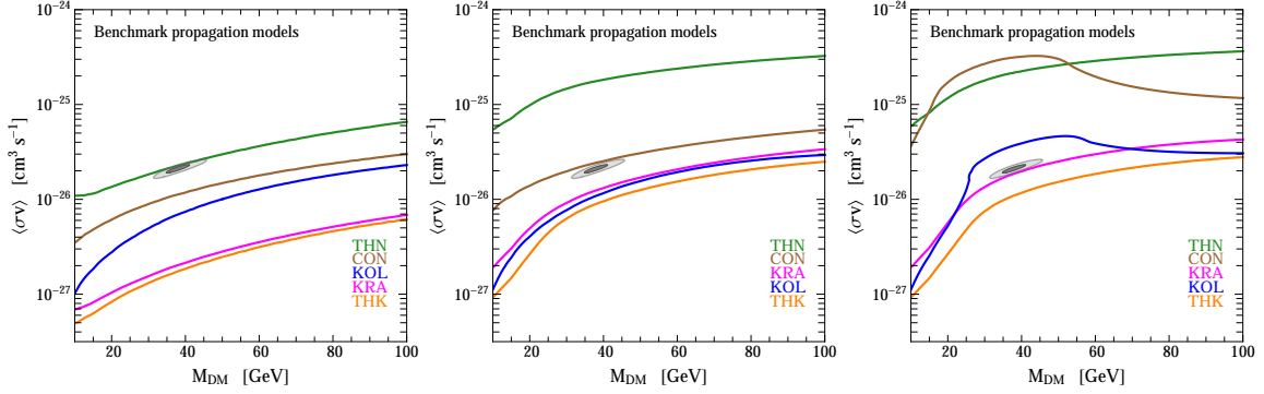
Figure 11: Antiproton constraints on the DM interpretation of the GC GeV excess, assuming fixed (left), flexible (middle) or essentially free (right) parameters for solar modulation (from [105] or [23]).
