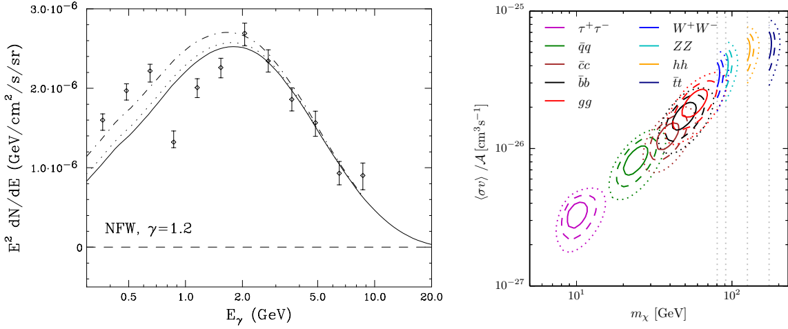
Figure 10: The GC GeV excess as seen in residual FERMI data (left, in the analysis of [86]) and its DM interpretation (right, from [91]).
