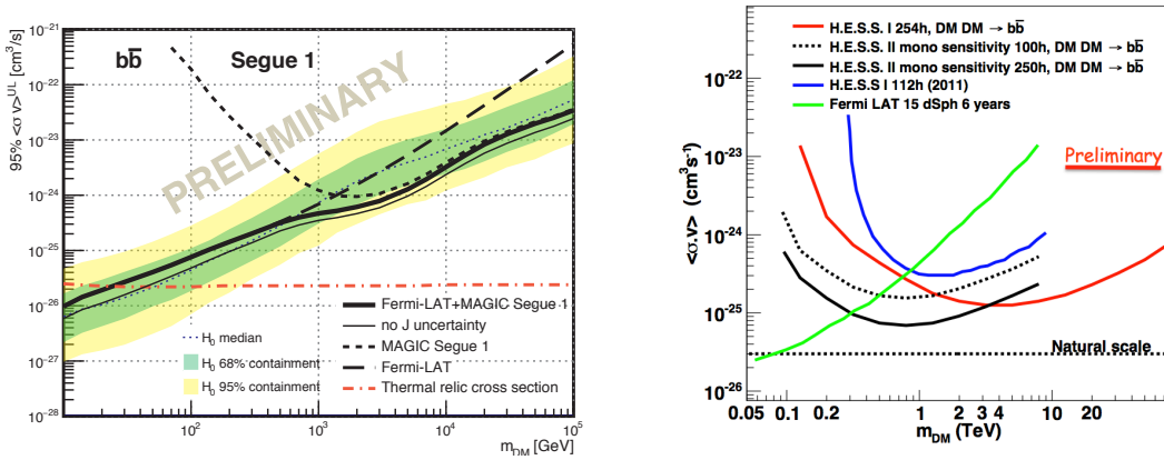
Figure 8: Two new results concerning \gamma -ray constraints on DM that have been presented at ICRC 2015: the bound by FERMI and MAGIC from the observation of dwarf galaxies (left, from [65]) and the bounds by HESS from the observation of the GC region (right, from [60]).
