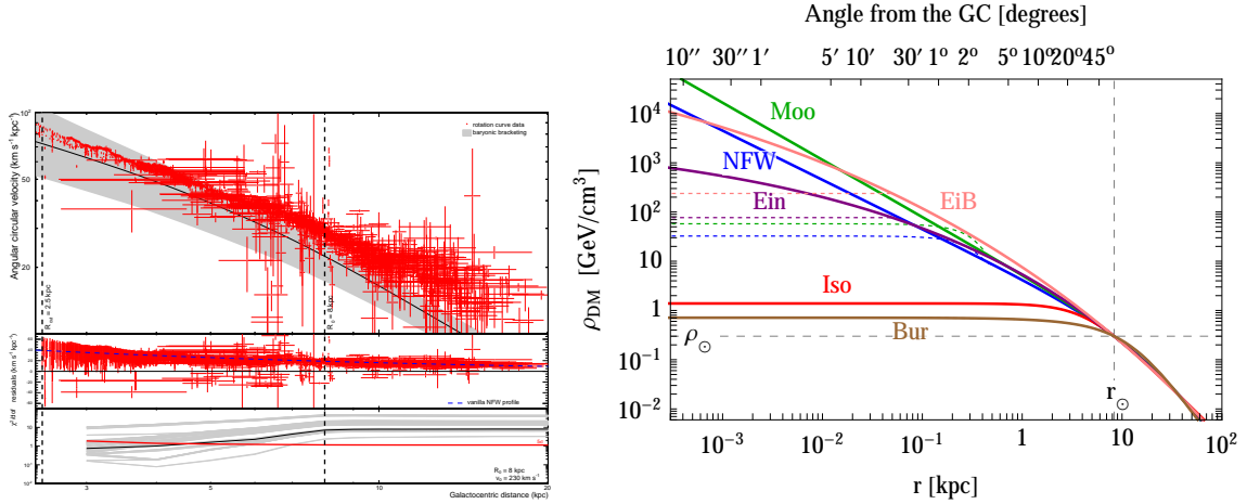
Figure 2: Left: a collection of galactic kinematical data and their use to claim evidence for DM in the Galaxy as well as, in principle, to determine its distribution (figure from [26, 27]). Right: an illustration of the most-often used DM profiles (from [29]).
