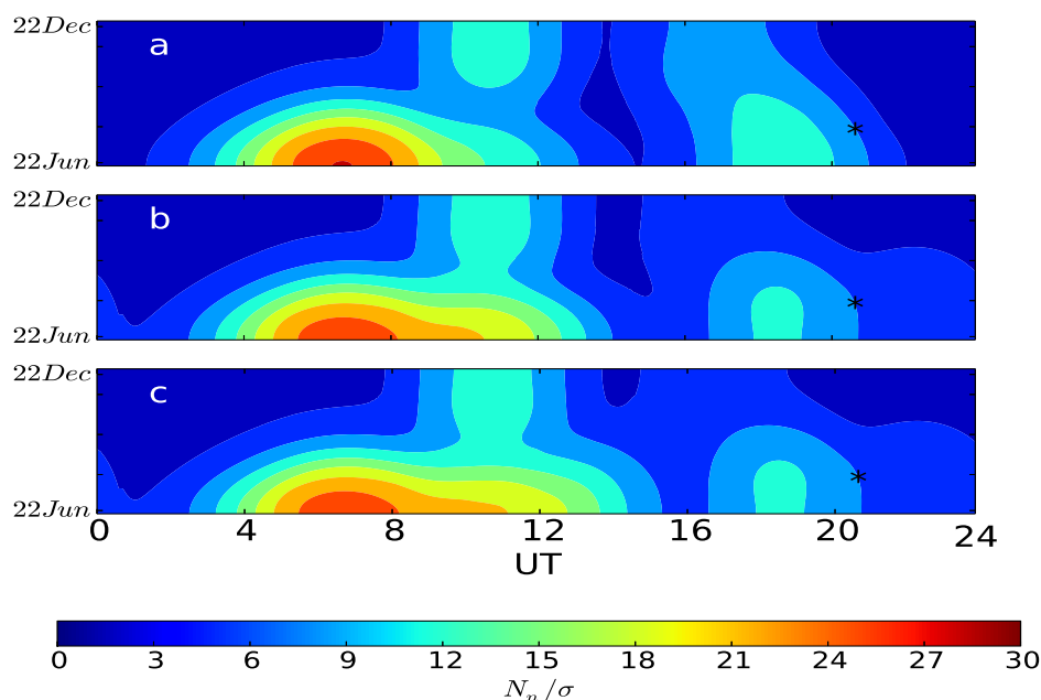
Figure 2: The sensitivity of the world neutron monitor network to an intense SNE similar to that of 24 May 1990 as a function of time of occurrence of the event. The real time of the event of 24.05.1990 is denoted by asterisk in the figure. a) The world NM network corresponding to the epoch 1990 b) The world NM network corresponding to the epoch 2010 c) The world NM for the epoch 2010 expanded with a 12NM64 at Canary islands.
