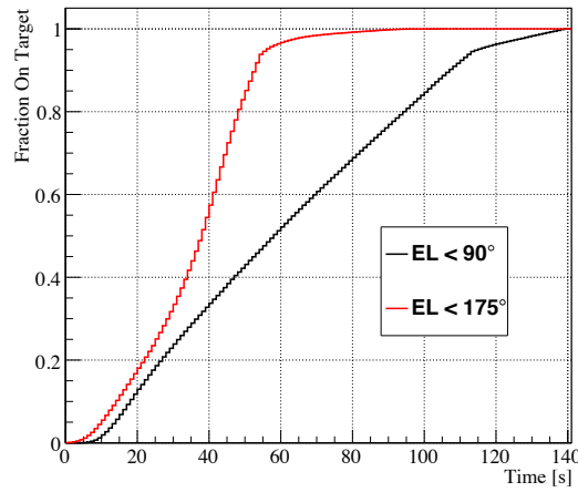
Figure 1: Fraction of times within which the CT5 telescope is able to arrive at a (random) target position on the sky versus the time after the issue of the repointing command. This fraction is shown for the systems with (elevation < 175°, red line) and without (elevation < 90°, black line) reverse-mode enabled. Figure reproduced from [8].
