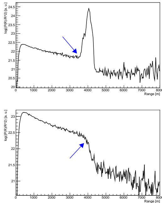
Figure 5: An example of a Raman and an elastic signals acquired by the ARCADE Lidar. A cloud is present above the lidar: it appears as a bump in the elastic signal (top) and as a drop in the Raman one (bottom).
