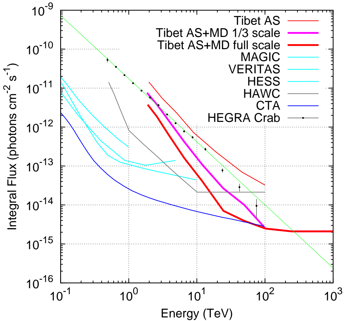
Figure 2: Expeced integral sensitivity to a gamma-ray point source of the Tibet AS+MD Project where AS area is assumed to be 37,000m 2 in this figure, together with various other experiments or projects.
