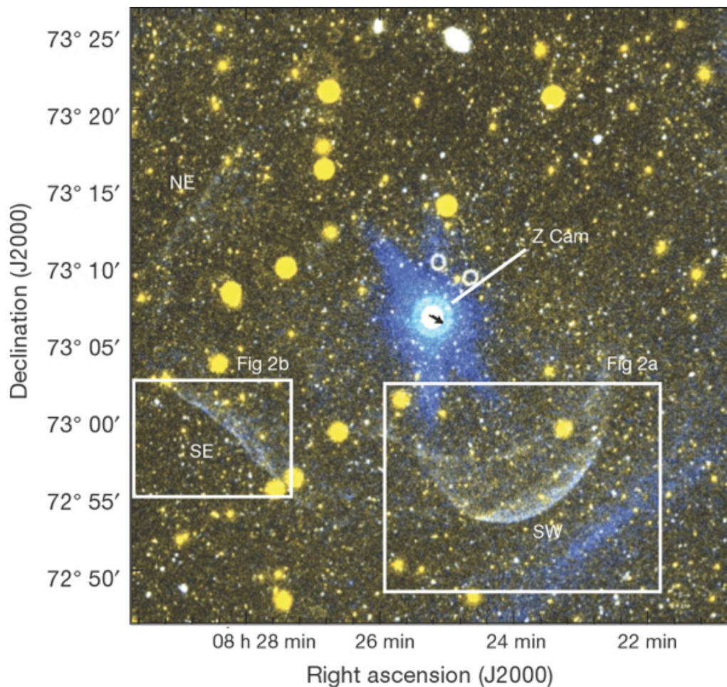
Figure 3: Figure from Shara et al (2007) highlighting the emission nebulosity around Z Cam.
