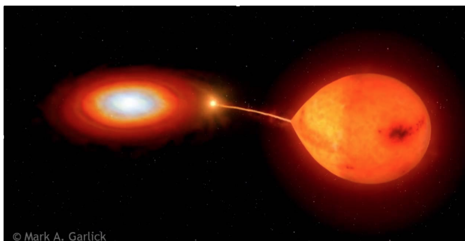
Figure 2: Artist's impression of a CV, copyright: Mark A. Garlick.
