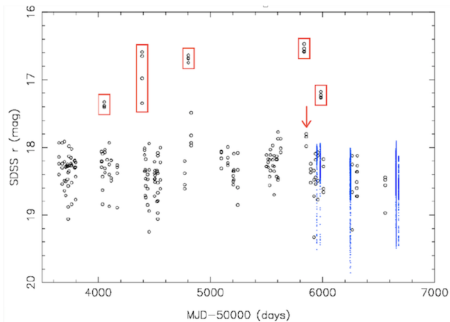
Figure 5: Figure from Drake et al (2009) highlighting the outbursts and eclipses of Te 11.
