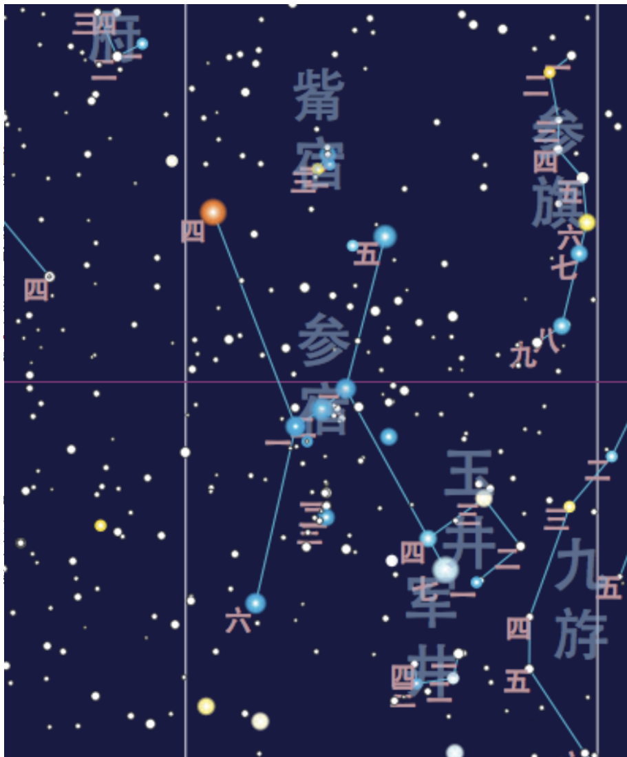
Figure 6: Image of the Three Stars mansion from the Chinese constellations (taken from Wikipedia).
