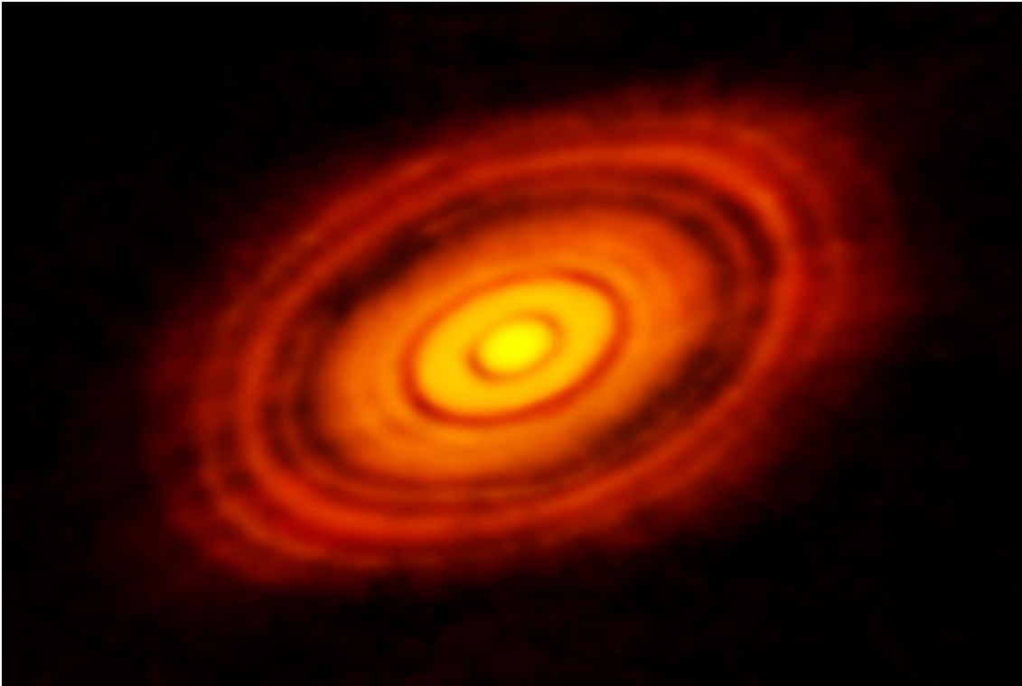
Figure 1: HL Tauri: note the ring-like structure that is likely to represent planetary formation in the protostellar system. This image is from ALMA (Atacama Large Millimeter/sub-millimeter Array).
