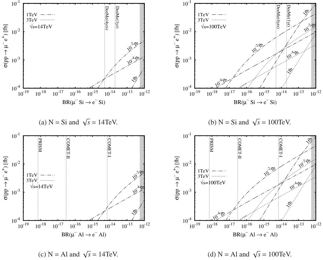
Figure 1: \sigma(pp \rightarrow \mu^- e^+) as a function of \text{BR}(\mu^- N \rightarrow e^- N) for each \sigma(pp \rightarrow jj) in the case-I. \sigma(pp \rightarrow jj) are attached on each line. Results for m_{\tilde{\nu}_\tau} = 1\text{TeV} ( m_{\tilde{\nu}_\tau} = 3\text{TeV} ) are given by dot-dashed (dotted) line. Shaded region is the excluded region by the SINDRUM-II experiment. Left and right panels show the results for \sqrt{s} = 14\text{TeV} and for \sqrt{s} = 100\text{TeV} , respectively. We take Si [(a), (b)], and Al [(c), (d)] for the target nucleus of \mu - e conversion.
