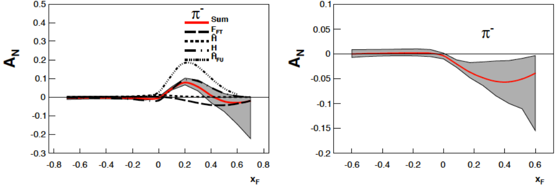
Figure 3: Prediction for A_N^{\ell N^\dagger \rightarrow \pi X} as function of x_F for \pi^- (left panel) and \pi^- (right panel with \hat{H}_{FU}^S = 0 ) production at P_{h\perp} = 3 GeV for typical EIC kinematics ( \sqrt{S} = 63 GeV).
