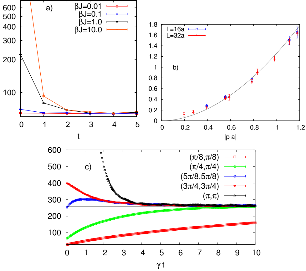
Figure 1: a) Real-time evolution of \langle M_s^2 \rangle driven by discrete measurements, for \beta J = 0.01, 0.1, 1, and 10 , for L = 16a . b) Inverse equilibration time 1/[\gamma\tau(p)] as a function of |p| for L = 16a, \beta J = 40 , and L = 32a, \beta J = 80 . c) Evolution of the Fourier modes \langle |\tilde{S}(p)|^2 \rangle for the Heisenberg anti-ferromagnet driven by a continuous Lindblad process. The initial ensemble is at a low temperature \beta J = 5L/2a , where a is the lattice spacing.
