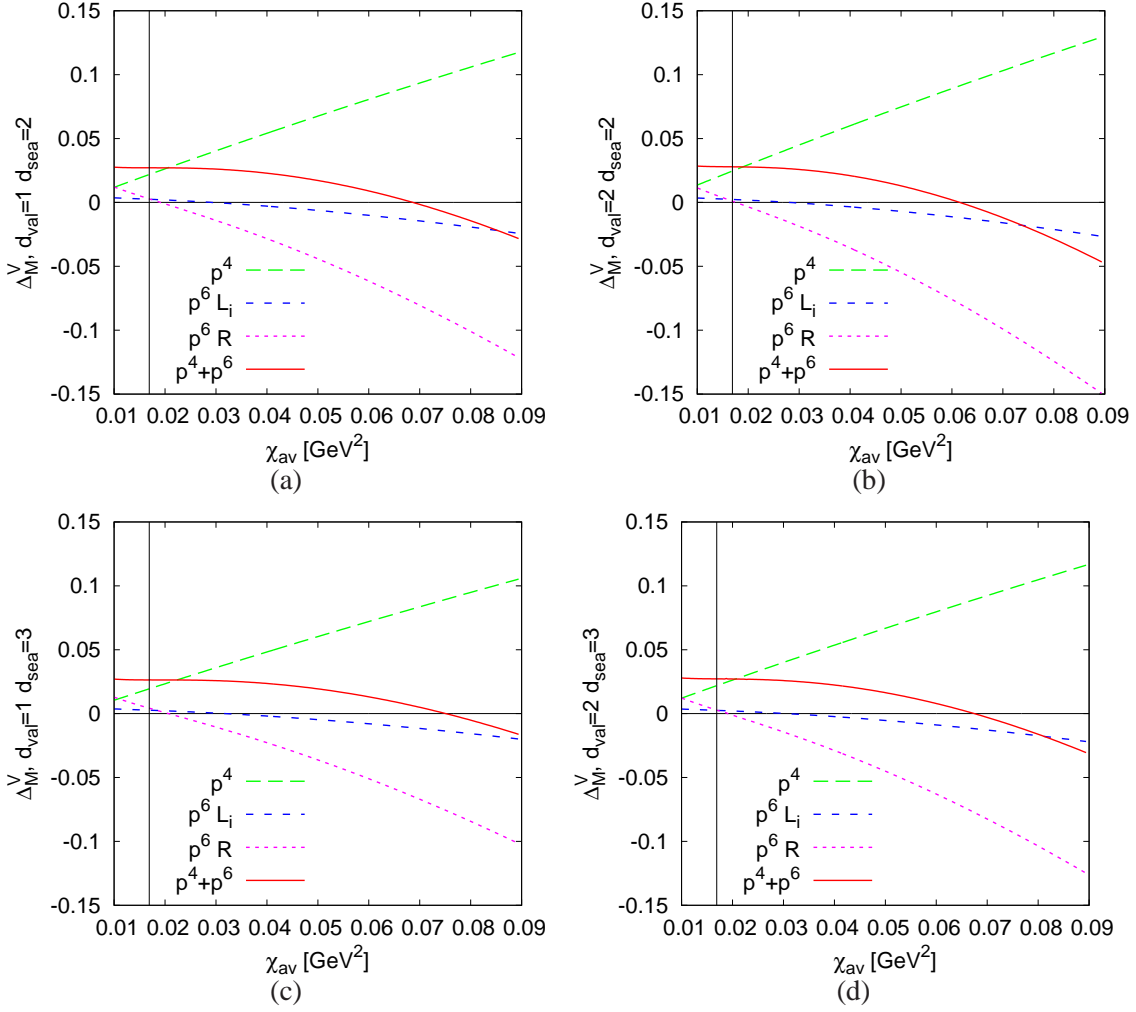
Figure 5: The corrections for the pion mass relative to the lowest order mass as a function of the average up and down sea quark mass via \chi_{av} . When isospin breaking is included the ratio of up to down quark mass is chosen to be 1/2 . d_{val} indicates the number of different valence quark masses, d_{sea} indicates the number of different sea quark masses. p^6 L_i denotes the part of the p^6 contribution depending on the L_i^r while p^6 R is the p^6 contribution which does not depend on p^4 or p^6 LECs. The vertical line at \chi_{av} = 0.0169 in this and the following figures indicates where the lowest order masses for the pion composed of sea quarks and of valence quarks are the same. This is the unquenched case for (a) and (d). (a) The isospin limit in sea and valence, (b) Isospin breaking in the valence sector only. (c) Isospin breaking in the sea sector only. (d) Isospin breaking in both sectors.
