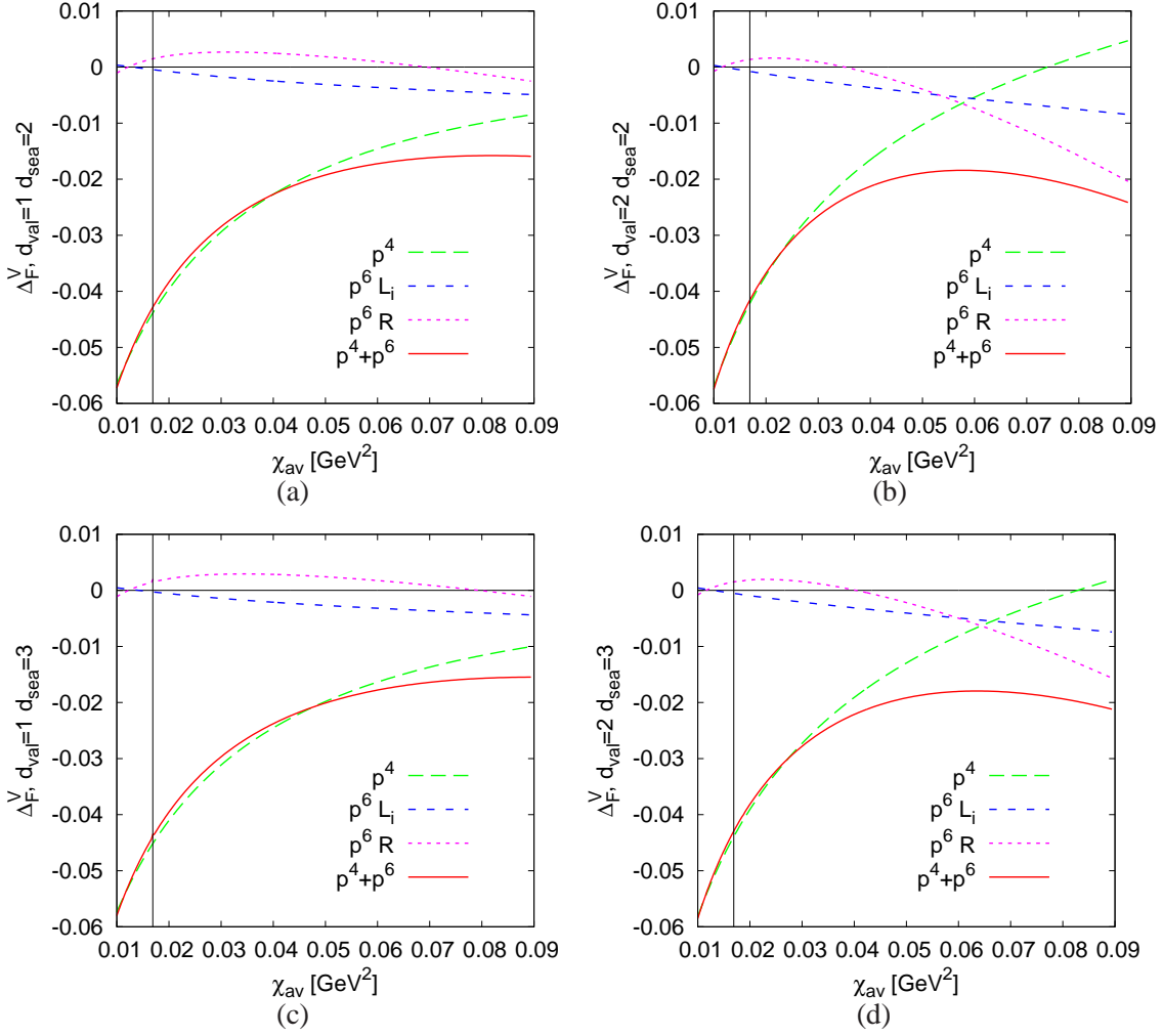
Figure 7: The corrections for the pion decay constant relative to its lowest order value as a function of the average up and down sea quark mass via \chi_{av} . (a) The isospin limit. (b) Isospin breaking in the valence sector. (c) Isospin breaking in the sea sector. (d) Isospin breaking in both sectors.
