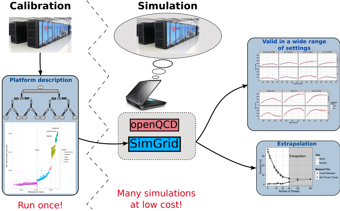
Figure 2: Workflow for coupling the openQCD package and SimGrid. Once platform characteristics have been benchmarked and network models have been instantiated, many simulations can be run at low cost to provide faithful predictions for a wide range of scenarios.
