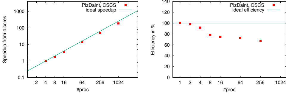
Figure 1: Strong and weak scaling of the ym1 program on a typical Cray machine (PizDaint, CSCS). Strong scaling plot shown in the left panel is obtained by running ym1 on a global lattice of a size 32^4 . Local lattice size used for the weak scaling plot shown in the right panel is 8^4 . Both plots are obtained with run parameters from the sample input file ym1.in distributed with openQCD [1].
