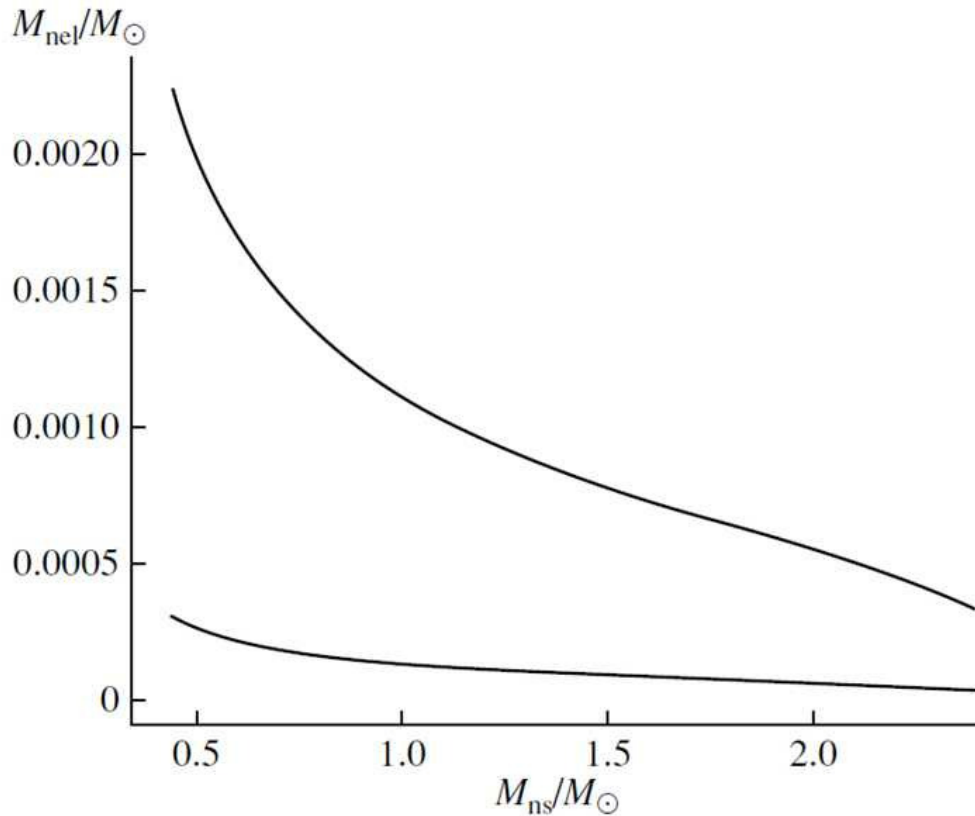
Figure 7: Dependence of the mass of the non-equilibrium layer on the neutron-star mass. The lines show the top and bottom boundaries of the layer mass measured from the stellar surface. The equation of state of the equilibrium matter [2, 54] was used to construct the model of the neutron star, with the boundaries of the layer specified by the densities. Using a non-equilibrium equation of state will increase the mass of the layer, but should not fundamentally change the values given in the figure, from Bisnovaty-Kogan (2012), calculated and prepared by S.O. Tarasov.
