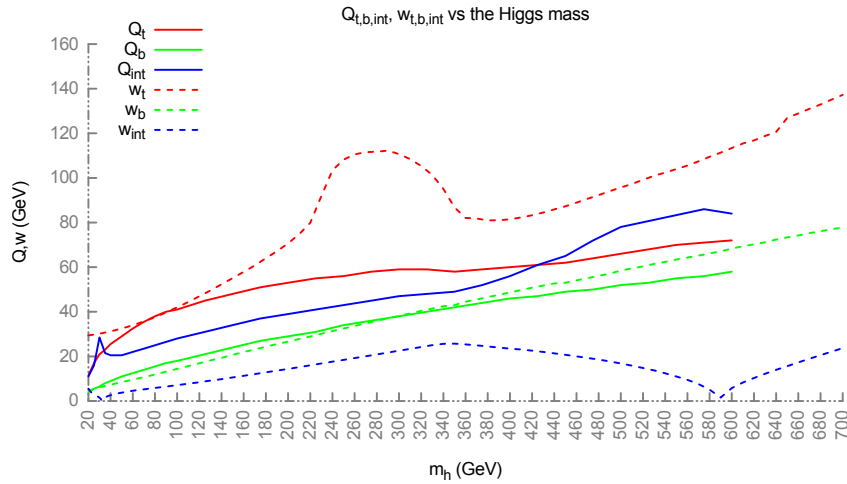
Figure 2: Comparison of the matching scales, for the top (red) and bottom (green) contributions and for the interference term (blue), obtained with either the BV ( w_i , dashed lines) or the HMW prescription ( Q_i , solid lines) as a function of the Higgs mass.
