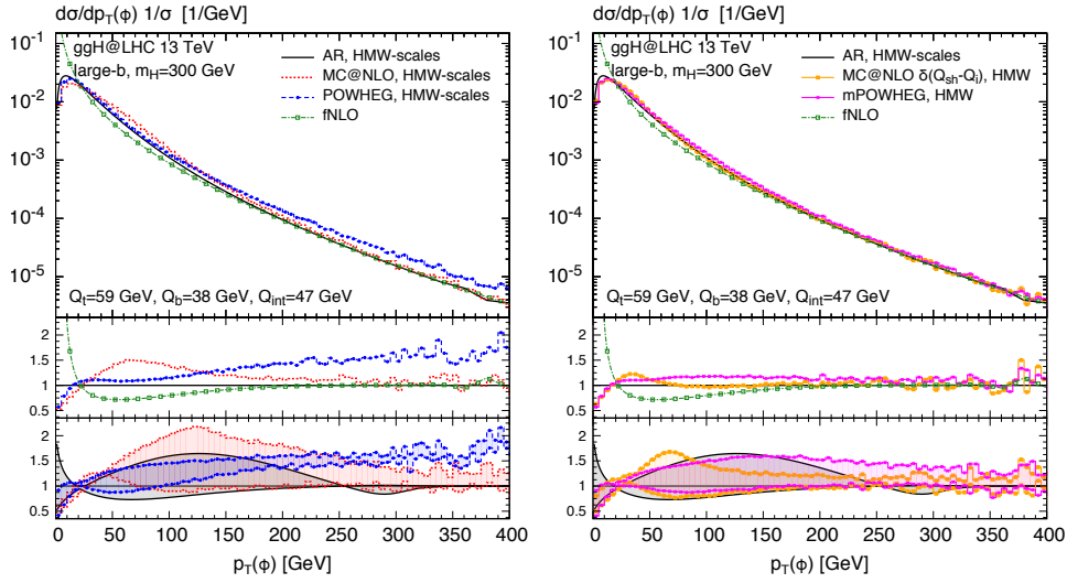
Figure 4: The plot on the left is as in fig. 3 but for the production of a heavy CP-even Higgs of m_H = 300 GeV and for the use of the HMW scales. On the right we show the results with the MC@NLO and POWHEG curves obtained with the changes to the shower scale prescription as described in the text.
