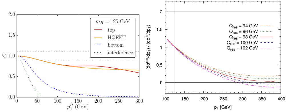
Figure 1: On the left, ratio ( C ) between the full squared matrix amplitude and the collinear limit of the gluon initiated subprocess for the top, bottom and interference terms as well as for the HQEFT computation, as a function of the Higgs transverse momentum; the dashed lines indicate a deviation of \pm 10\% from one. On the right, ratio between the matched and the fixed order predictions at the hadronic level, for the top contribution and for different values of matching scale. The latter is here denoted by Q_{\text{res}} because the results shown are obtained in the framework of AR.
