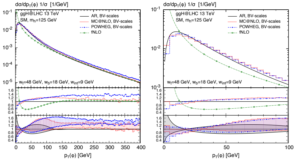
Figure 3: Shapes of the transverse momentum distribution for a SM Higgs boson of mass m_h = 125 GeV. We show the curves from AR (black, solid), MC@NLO (red, dotted) and POWHEG (blue, dashed overlaid by points) for the BV scale set. For reference we also show the fixed order result (green, dash-dotted with open boxes). On the left, we plot the spectrum up to 400 GeV, on the right we show a zoom around the first 100 GeV. In the main frame we show the absolute distributions, in the middle inset the ratio of the central curves to the analytic resummation result and in the bottom inset the uncertainty bands, again normalized to the AR resummation value.
