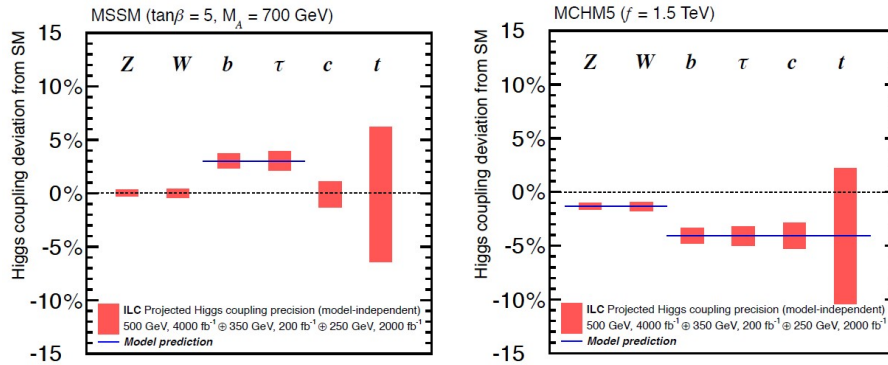
Figure 1: Examples of how new physics models can change the pattern of Higgs boson couplings [4].
