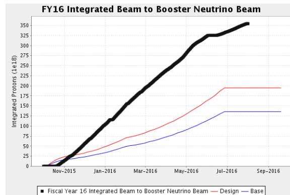
Figure 3: Integrated protons on target (black) to BNB compared to base (blue) and design (red) goals since October 2015.
