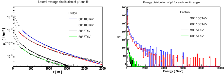
Figure 1: Number of muons per m^2 (left) and energy spectra of muons expected in surface (right) for proton as primary particle. Fe results are similar and could be find at Ref. [10].
