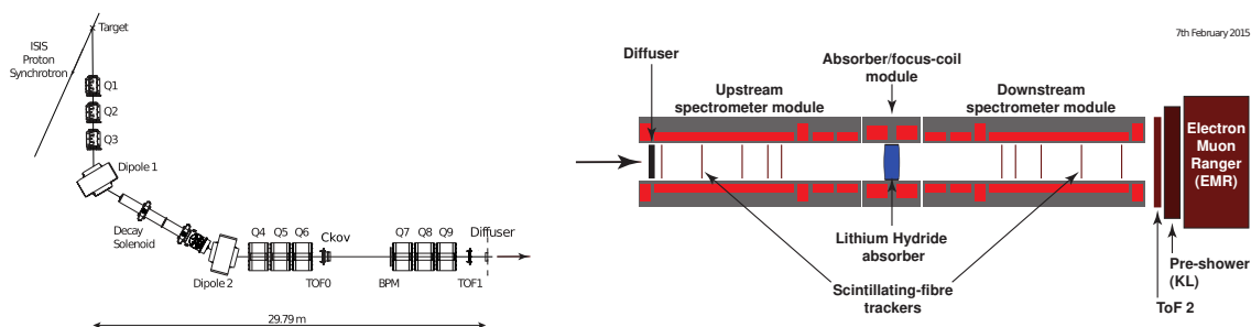
Figure 2: Layout of the MICE beamline (left) and cooling channel (right) in its current configuration. The solenoid magnet coils are marked in red and the absorber module is shown in blue.
