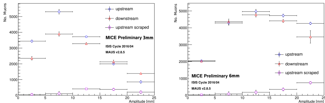
Figure 5: A comparison between the upstream and downstream amplitude distributions for the 3 mm nominal beam and the 6 mm nominal beam. The particles that were reconstructed upstream but were scraped before reaching the downstream tracker are also shown.
