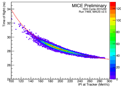
Figure 4: Comparison of the time of the flight between TOF0 and TOF1 and the momentum reconstructed within the upstream tracker. The red dashed line describes the theoretical results for a particle with the muon mass.
