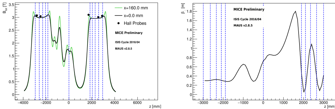
Figure 3: The magnetic field configuration (left) and betatron function from simulation (right) that was used during data taking. The blue dashed lines highlight the positions of the 5 tracker stations, upstream and downstream, in addition to the centre of the LiH absorber. The green line shows the magnetic field strength at the radius of the hall probes.
