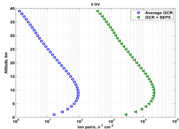
Fig. 5. Ion pairs profiles during GLE05 (or SEP05) on 23.02.1956 for geom. cut-off 5 GV.
