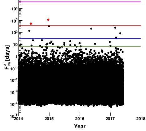
Figure 7: Distributions of detected clusters versus time for the present data set. Red dots represent clusters with imitation frequency less than F_{im} = 1/\text{year} . Green, blue, red and purple lines corresponds to F_{im}^{\text{th}} = 1/\text{week} , F_{im}^{\text{th}} = 1/\text{month} , F_{im}^{\text{th}} = 1/\text{y} , F_{im}^{\text{th}} = 1/100 \text{ y} , respectively
