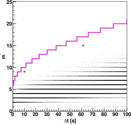
Figure 6: Distribution of detected clusters in the space (\Delta t, m^*) . Red dots represent clusters with imitation frequency less than F_{im} = 1/\text{year} . The purple line corresponds to F_{im}^{\text{th}} = 1/100 years.
