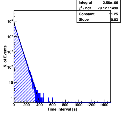
Figure 3: Distribution of normalized time intervals between triggers of the last run.
