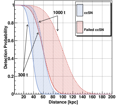
Figure 5: LVD detection probability versus source distance for the F_{im} = 1/100 \text{ yr}^{-1} for both ccSN and failed supernovae in the range of minimum (300 t) and maximum (1000 t) allowed active mass.
