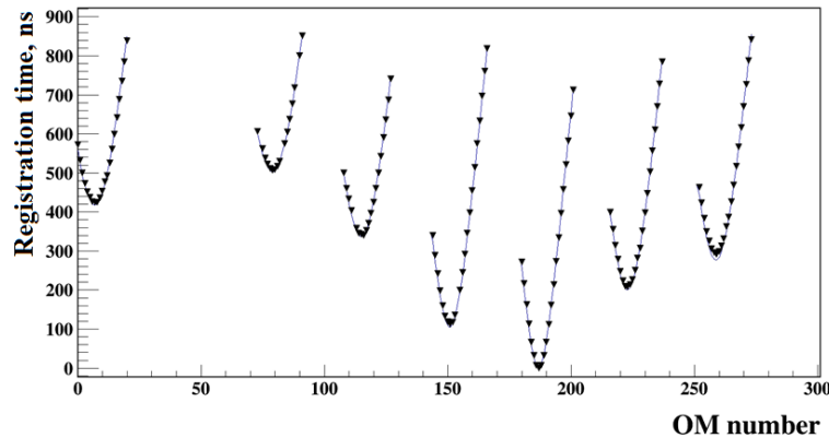
Fig. 4.2. An example of a laser event detected with the cluster of Baikal-GVD.
