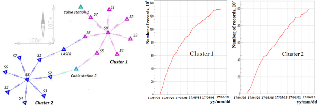
Fig. 4.1. Layout of the installation and accumulative number of the master records detected with two clusters (since April 13 to June 15 of 2017).
