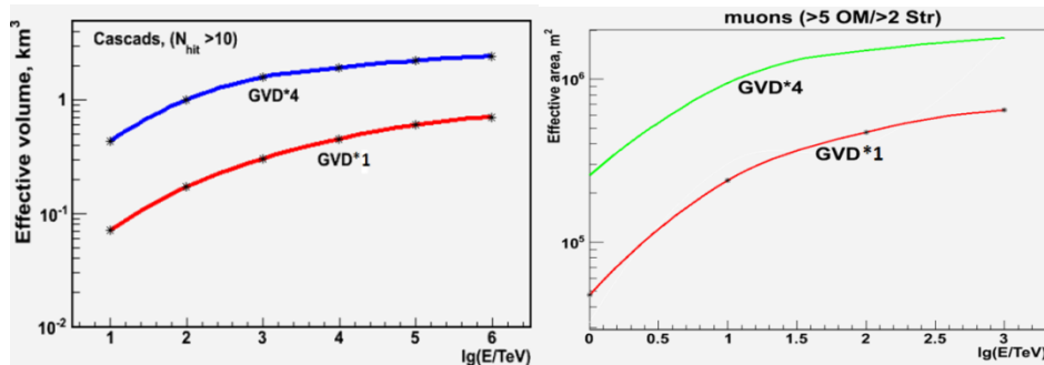
Fig. 2.2. The effective volume for the registration of the cascades and the effective area for muons depending on the energy for GVD-1 and full-scale neutrino telescope Baikal-GVD (GVD-4).
