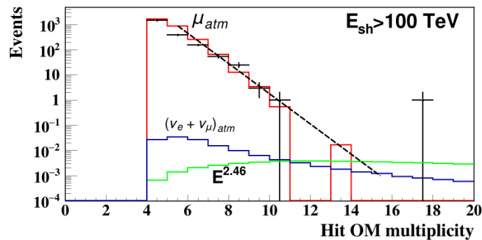
Fig. 5.1. The distribution of cascade-like events with energies above 100 TeV on the multiplicity of hit channels; points - experiment, red line - background of atmospheric muons, blue line - background of atmospheric neutrinos, green line - expected signal from astrophysical neutrinos.
