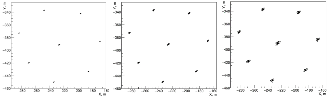
Fig. 4.3. The results of the measurement of the position of the acoustic modems installed on the eight strings of the cluster for different distances from AM to the string bottom: z = 181 m (left), z = 346 m (center), z = 538 m (right).
