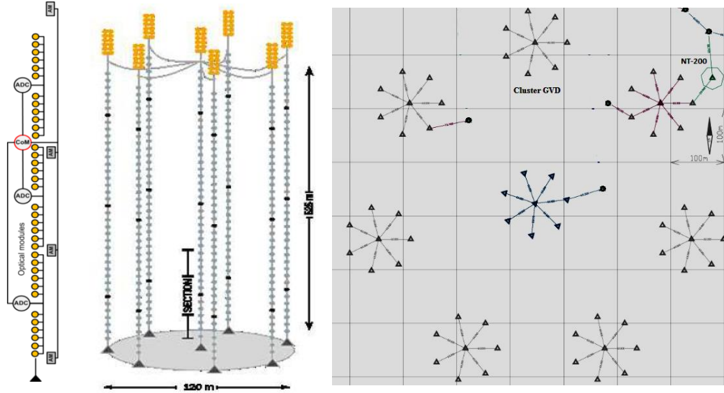
Fig. 2.1. Block diagram of the string and view of the cluster Baikal-GVD (left), and layout of eight clusters of the GVD-1 (right).
