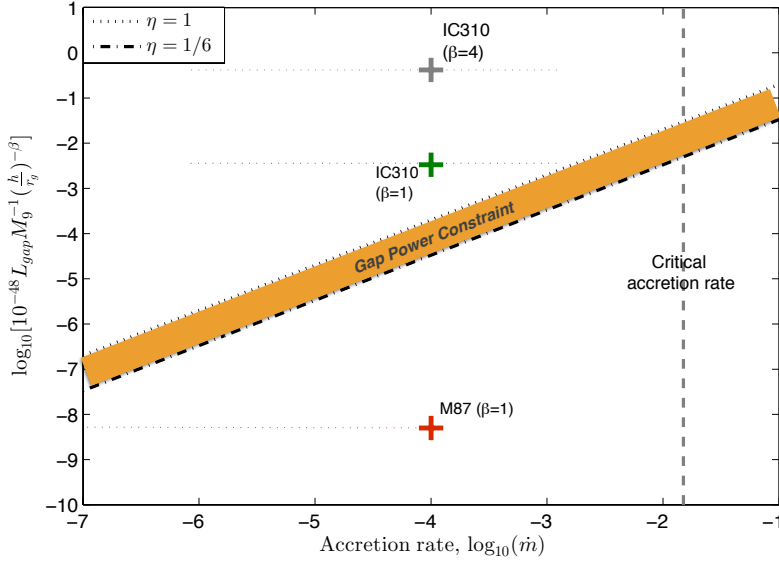
Figure 2: Maximum possible gamma-ray power (orange band) of a magnetospheric gap as a function of accretion rate, cf. eq. (3.5). Different assumptions on the gap potential, eqs. (3.3)–(3.4), lead to a difference in extractable powers. The required transparency of the accretion environment to VHE photon introduce an upper limit \dot{m}_c \simeq 0.01 on possible rates. If the observed VHE variability is used to constrain the gap height h , the extractable power is in principle sufficient to account for the gamma-ray emission seen from M 87 , yet under-predicts the VHE emission seen from IC 310 . See ref. [8] for further details.
