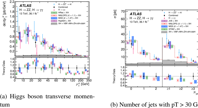
Figure 1: Differential cross sections in the full phase space measured with the H \rightarrow \gamma\gamma (red upward triangle) and H \rightarrow ZZ^* \rightarrow 4\ell (blue downward triangle) decay channels, as well as the combined measurement (black circle). Different SM predictions are overlaid as colored points, with the colored boxes indicating their uncertainties.
