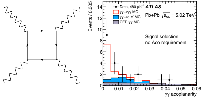
Figure 2: Left: Feynman diagram for direct light-by-light scattering. Right: Acoplanarity dependent cross sections for light-by-light scattering, compared to a SM calculation and known background contributions from misidentified electrons, and central exclusive production. Results from Ref. [9].
