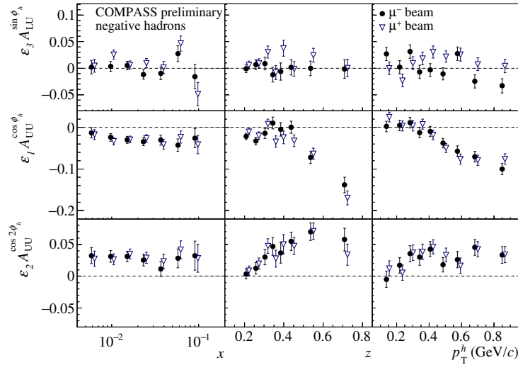
Figure 5: Azimuthal asymmetries for negative hadrons for the samples of data collected with positive and negative muon beams. Uncertainties are statistical only.
