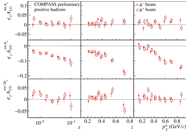
Figure 4: Azimuthal asymmetries for positive hadrons for the samples of data collected with positive and negative muon beams. Uncertainties are statistical only.
