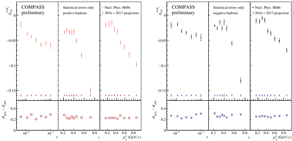
Figure 7: Comparison of \cos \phi_h asymmetry projected uncertainty for the whole 2016 and 2017 data with the published one [7], for positive and negative hadrons.
