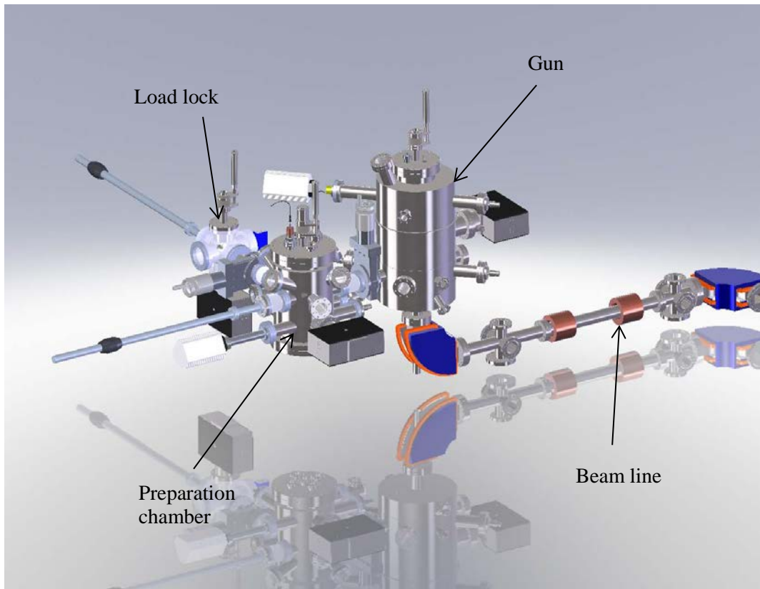
Figure 1. Gun and beam line layout.
