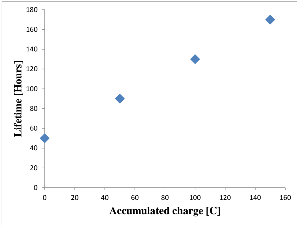
Figure 3. Lifetime at 1 mA beam current as a function of accumulated charge
