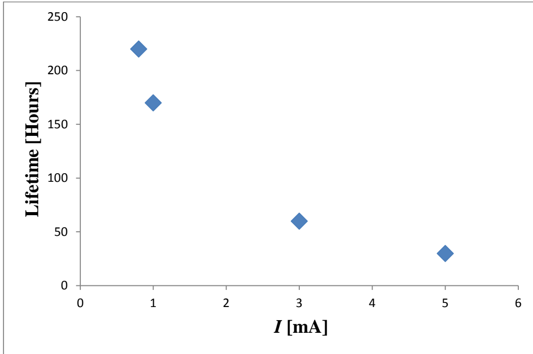
Figure 2. Lifetime measurements in mA range
