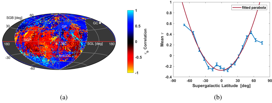
Figure 4: Seven year data result. (a) Projection of the correlation strength \tau_b for all grid points. Negative correlations expected for magnetic deflections are apparent around the supergalactic plane. Solid curves indicate the galactic plane (GP) in blue and supergalactic plane (SGP) in red. White and grey hexagrams indicate the Galactic center (GC) and anti-galactic center (Anti-GC) respectively. (b) Mean \tau_b inside equal solid angle bins. The correlation curvature is a=2.4 \times 10^{-4} .
