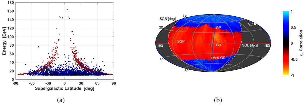
Figure 3: Toy-model supergalactic magnetic sheet simulation of anisotropic energies. (a) Blue circles are isotropic events ( F = 65.7\% ). Red squares are anisotropic events magnetically diffused away from the supergalactic plane with S \times B = 18.47 \text{ kpc} \times \mu\text{G} . All event positions are isotropic and the energy spectrum is created according to the published TA results. (b) Projection of the energy-angle correlation strength \tau_b inside wedges for all grid points. Solid curves indicate the galactic plane (GP) in blue and supergalactic plane (SGP) in red.
