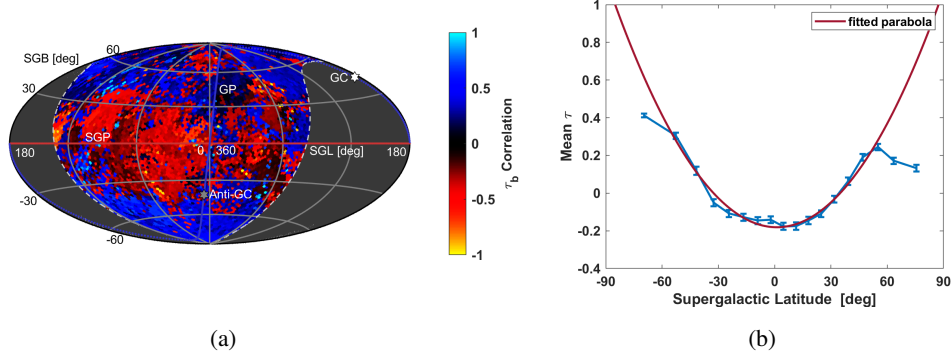
Figure 5: 10 year data result. (a) Projection of the correlation strength \tau_b for all grid points. Negative correlations expected for magnetic deflections are apparent around the supergalactic plane. (b) Mean \tau_b inside equal solid angle bins. The correlation curvature is a=1.6 \times 10^{-4} .
