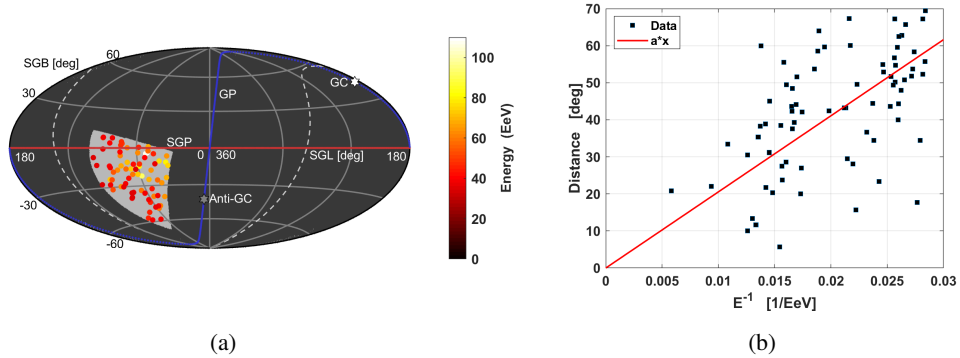
Figure 2: (a) Supergalactic Hammer-Aitoff projection of the 10 year maximum significance “wedge” at 30.3^\circ SGB, -3.2^\circ SGL. The correlation \tau_b = -0.412 with 75 data events has a pre-trial one-sided significance of 5.10\sigma . This increased from 4.58\sigma at this grid point with 7 years of data. The energy threshold is E_i \geq 35 EeV, wedge width W_i = 90^\circ , angular distance D_i = 70^\circ , and direction \phi_i = 120^\circ . (b) Scatter plot of 1/E_j versus angular distance \delta_j in the wedge.
