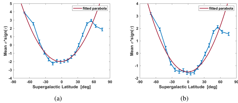
Figure 6: The mean sign(\tau_b) \times \sigma inside equal solid angle bins of SGL. (a) Seven years of data with a curvature parameter a = 0.0013 . (b) Ten years of data with a curvature parameter a = 0.0010 .
