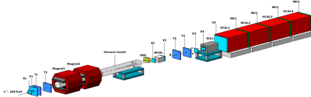
Figure 4: Setup of NA64 for the visible decay channel search of A' , X(17 \text{ MeV}) \rightarrow e^+e^- [7].
