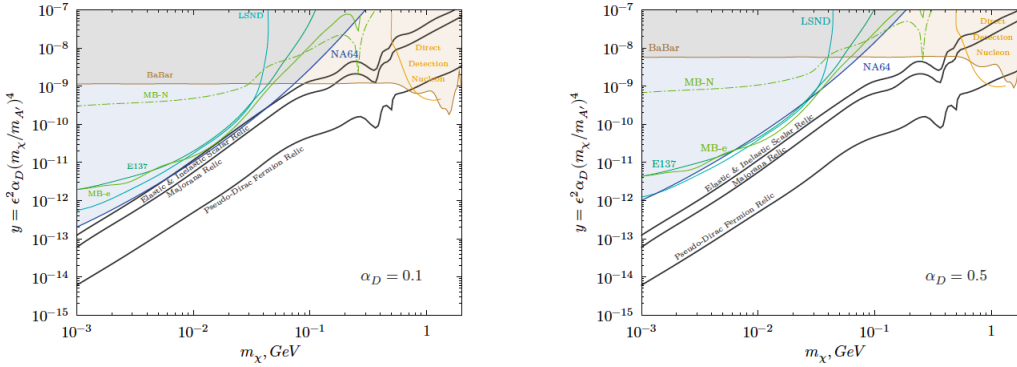
Figure 3: The NA64 sensitivity limits in the (M_\chi, y) plane along-with the limits from other experiments [4].
