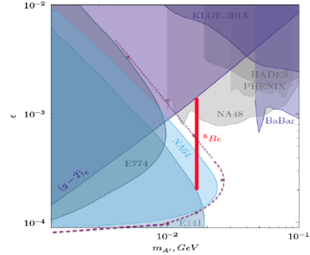
Figure 5: The A' parameter space excluded by the NA64 visible data of 2017 (blue shadowed region) and 2017+2018 (dashed line). The red vertical line is the region that could explain the ^8\text{Be} anomaly [4].
