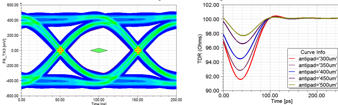
Figure 5. Simulated eye diagram of the lines between the Samtec FireFly and the Kintex UltraScale FPGA (left). Results of the TDR simulations of a differential via structure for different anti-pad diameters (right).
