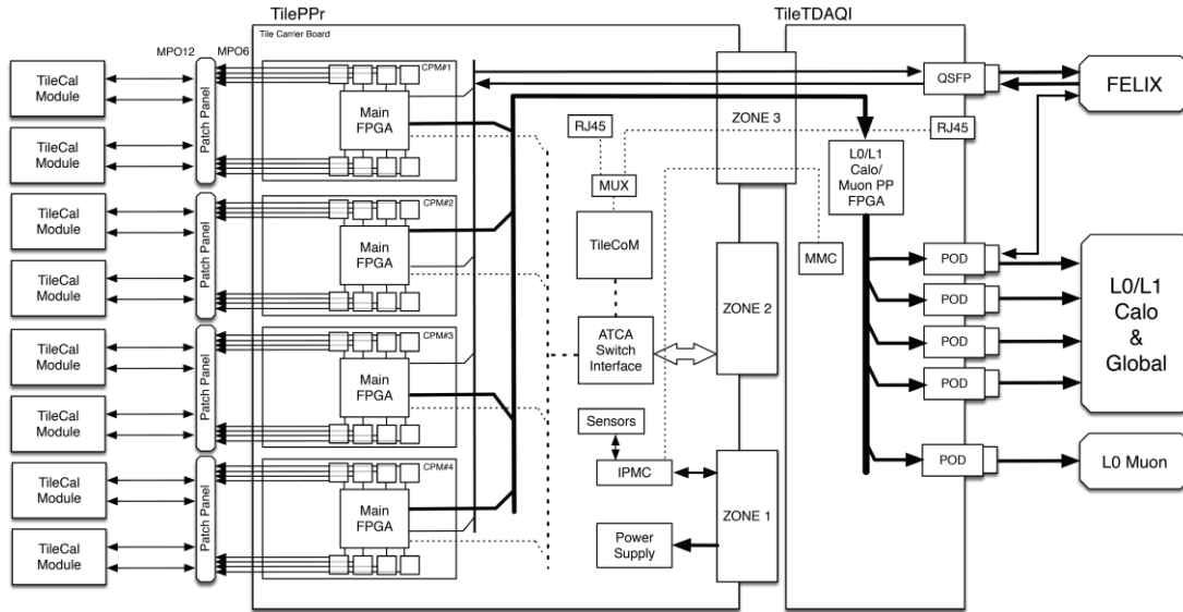
Figure 2. Block diagram of the TilePPr module.
