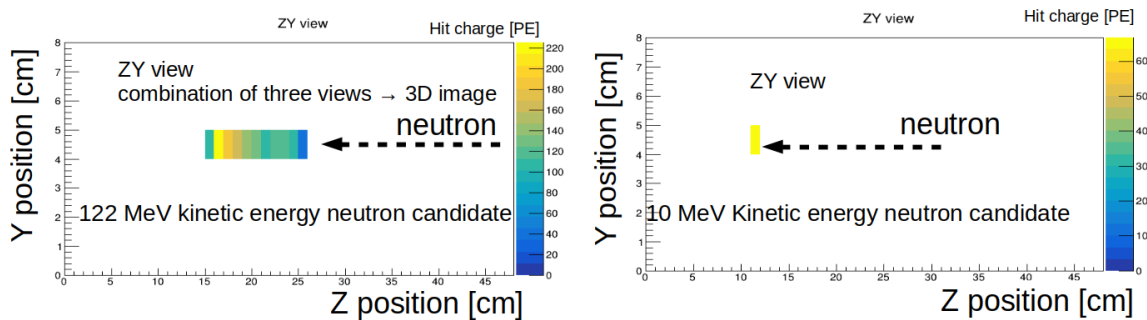
Figure 2: Two neutron-induced candidates on one of the three views in the superFGD prototype. The deposit energy can be calculated from the number of collected photoelectrons and it is less than the neutron kinetic energy.
