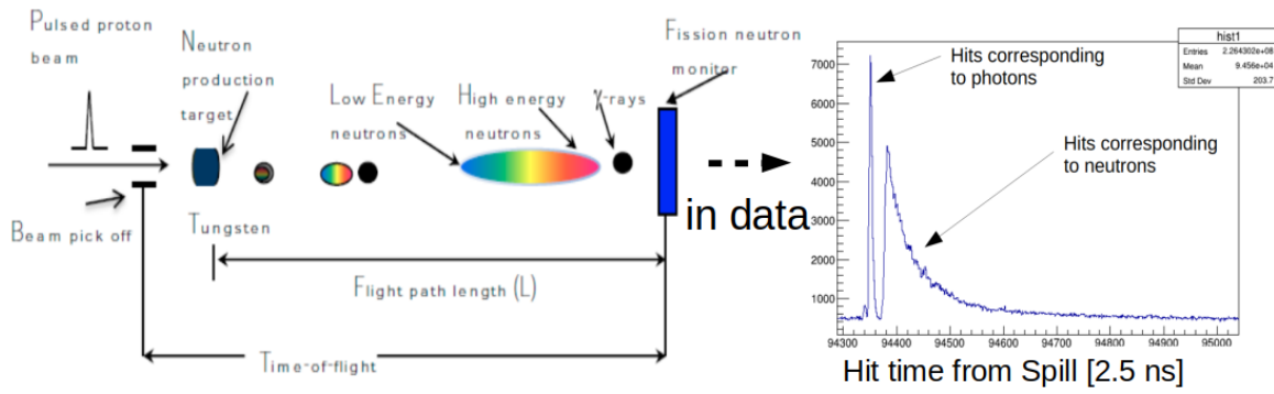
Figure 1: The principle of measuring neutron energy with time-of-flight and the time distribution measured in the detector.
