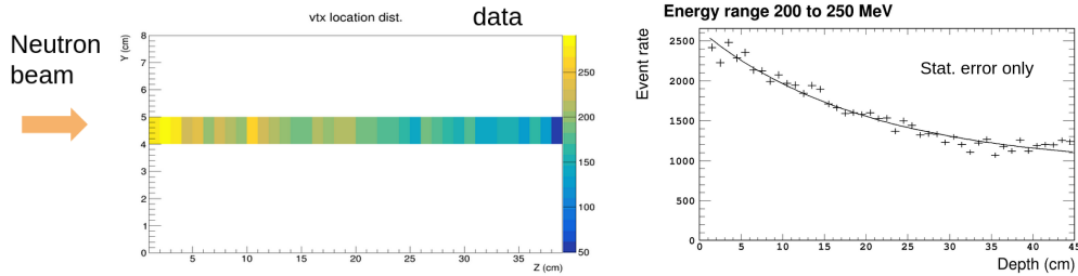
Figure 3: Left: vertex locations on depth of all neutron interactions on the YZ plane. Right: Single-track event rate along the depth layer for incident 200-250 MeV KE neutrons with an exponential fit.
