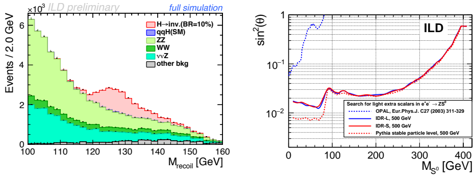
Figure 1: Left: recoil mass distribution after event selection for ILC running at 250 GeV and invisible Higgs branching ratio of 10% [1]. Right: expected sensitivity of the International Large Detector (ILD) experiment at the ILC, for ILC running at 500 GeV to the scalar sector mixing parameter \sin^2 \theta [3].
