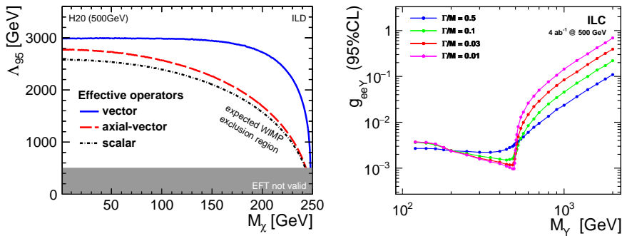
Figure 2: The expected sensitivity of the ILC experiment, for ILC running at 500 GeV, to DM pair production. Left: EFT limits on mediator mass scale \Lambda as a function of the DM particle mass M_\chi , for different mediator types [4]. Right: mediator coupling limits as a function of the vector mediator mass M_\gamma for DM particle mass M_\chi=50 GeV [5].
