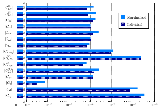
Figure 2: Constraints on C/\Lambda_{\text{CLFV}}^2 [GeV ^{-2} ] based on the current Belle limits, stemming from the marginalized and individual analyses for \tau decays, given at the 99.8% confidence level.
