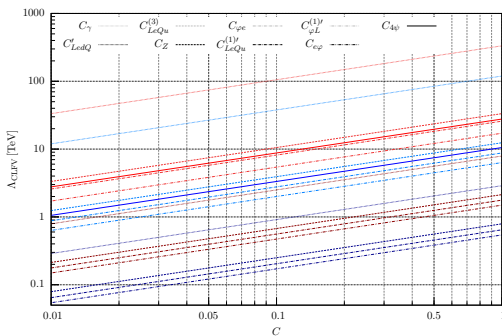
Figure 1: Constraints on \Lambda_{\text{CLFV}} with respect to the values of WCs, based on the current Belle (shades of blue) and expected Belle II (shades of red) limits, given at the 99.8% confidence level.
