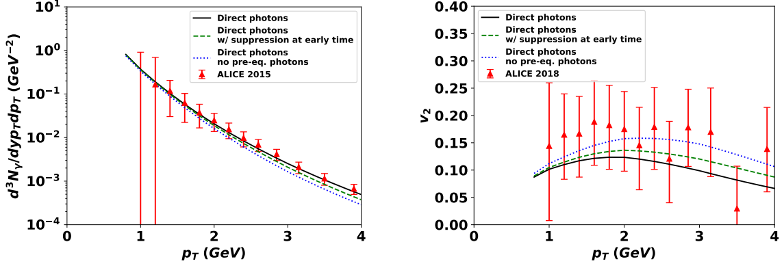
Figure 2: Direct photon yield and \nu_2 within 20 – 40% centrality for \sqrt{s_{NN}} = 2.76 TeV Pb-Pb collisions carried out at the LHC [5].
