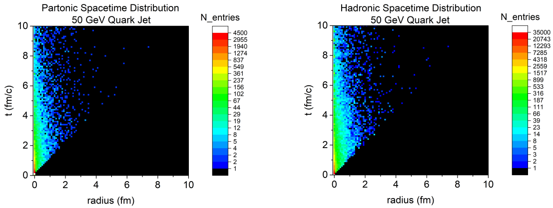
(a) The spacetime distribution of partons ready for hadronization ( Q < Q_0 = 1 GeV) in a 50 GeV quark jet in vacuum.
