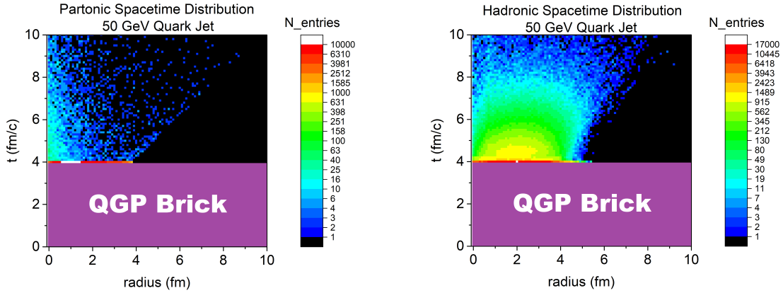
(c) The spacetime distribution of partons ready for hadronization ( Q < Q_0 = 1 GeV and T < T_C ) in a 50 GeV quark jet in a 4 fm brick.
