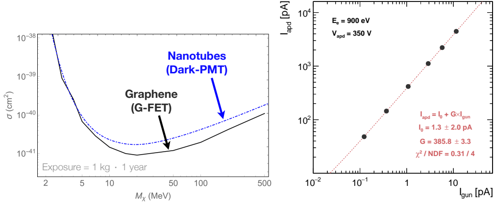
Figure 6: Left: Expected 90% cross section exclusion with an exposure of 1 \text{ kg} \times 1 \text{ year} for the G-FET concept (black) and the dark-PMT concept (blue dashed). Right: APD characterization carried out in LASEC laboratories in University of Roma Tre: APD current ( I_{apd} ) as a function of the electron gun current ( I_{gun} ).
